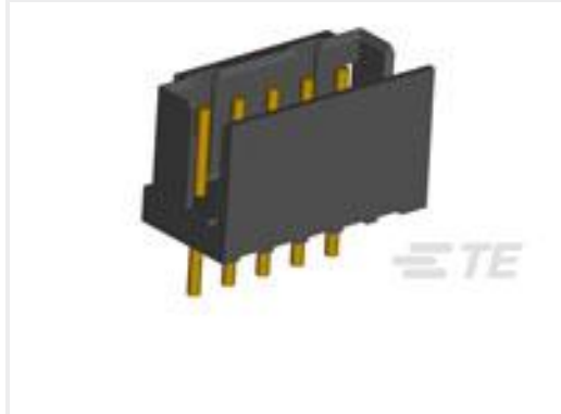
TE Part #1-292133-0 CT P/HDR ASSY BOX V 10P W/O KI
