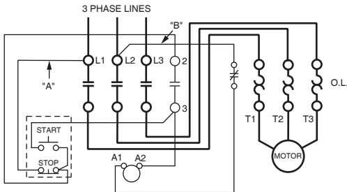
SEPARATE CONTROL CIRCUIT
