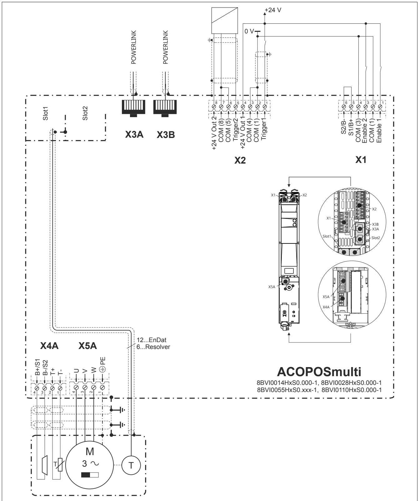
Figure 6: 8BVI0014HxS0.000-1, 8BVI0028HxS0.000-1, 8BVI0055HxS0.xxx-1, 8BVI0110HxS0.000-1 - Pinout overview
