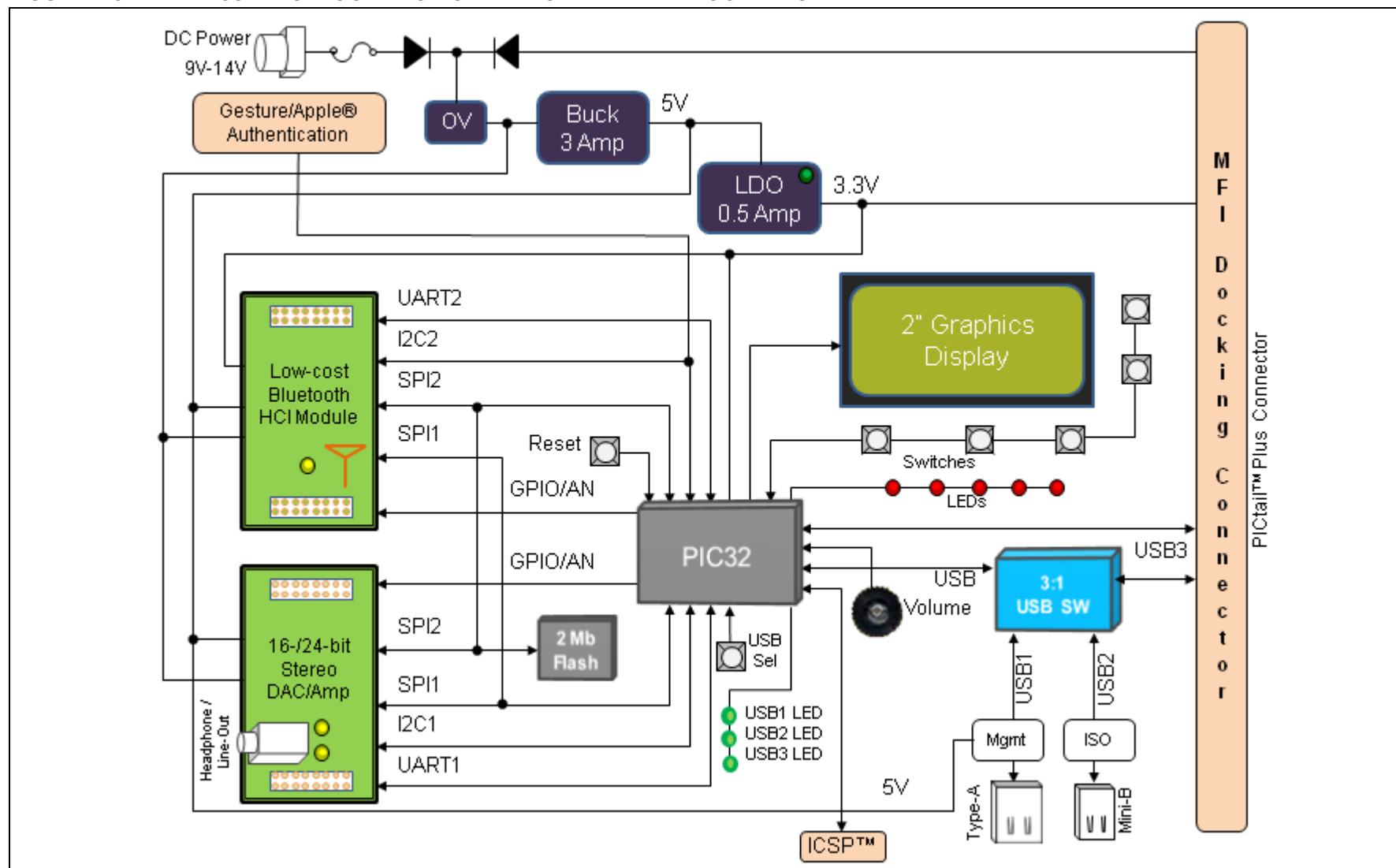
FIGURE 1-3: PIC32 BLUETOOTH AUDIO DEVELOPMENT KIT BLOCK DIAGRAM
