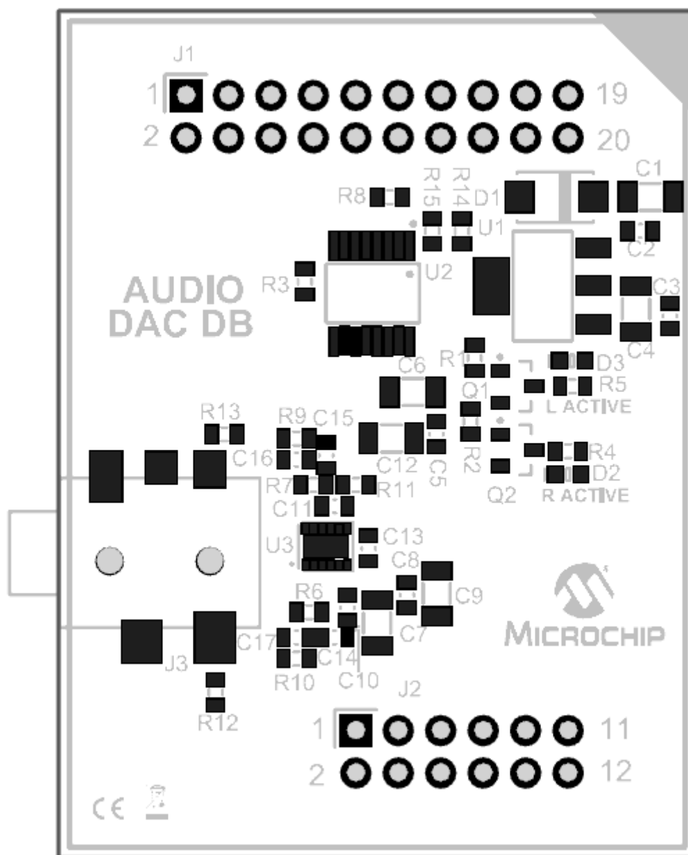
FIGURE A-4: AUDIO DAC/AMP DAUGHTER BOARD LAYOUT (TOP ASSEMBLY)
