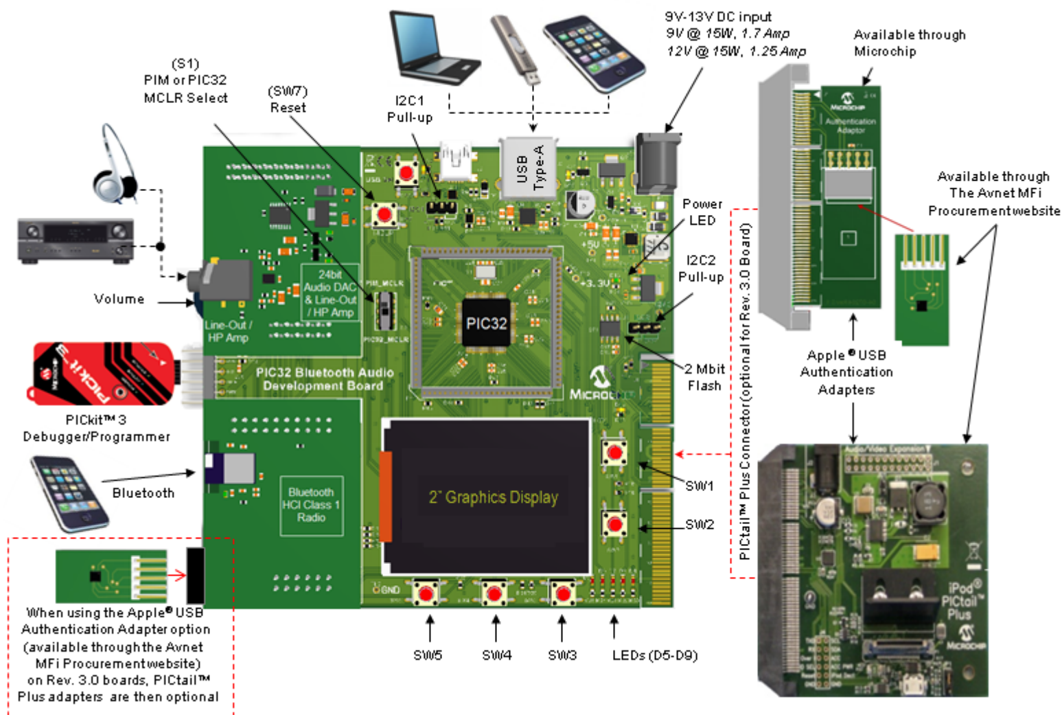
FIGURE 1-2: PIC32 BLUETOOTH AUDIO DEVELOPMENT KIT LAYOUT AND FEATURES
