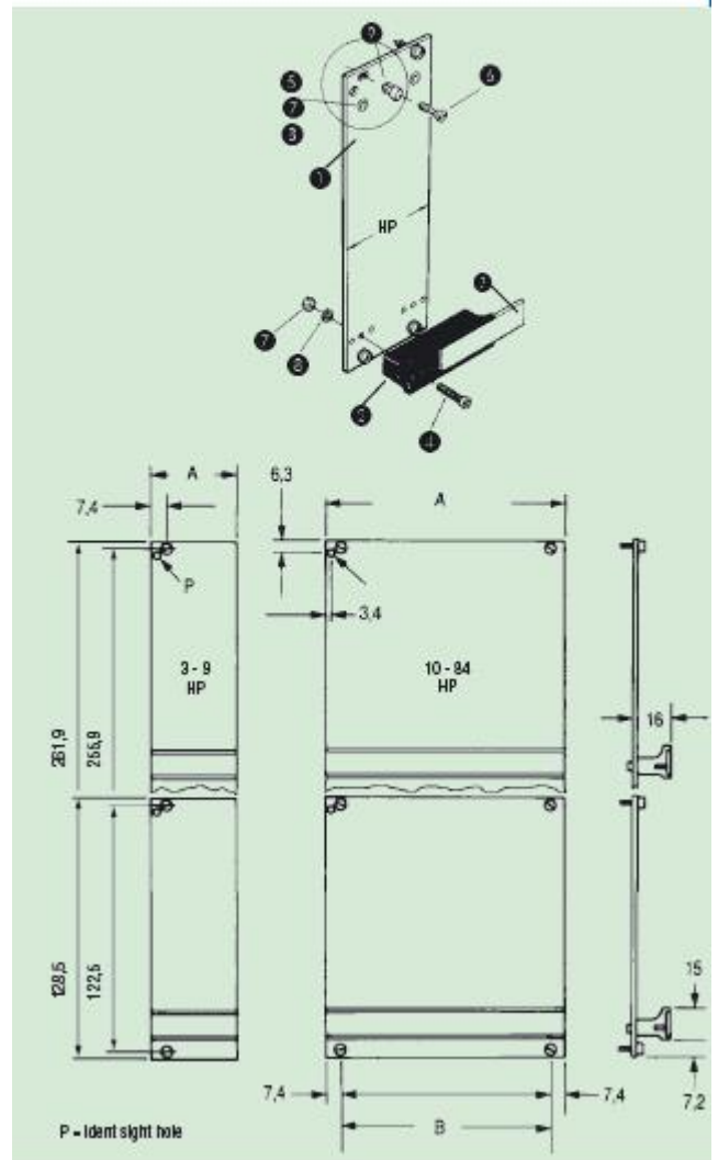
Standard 3U & 6U front panels
