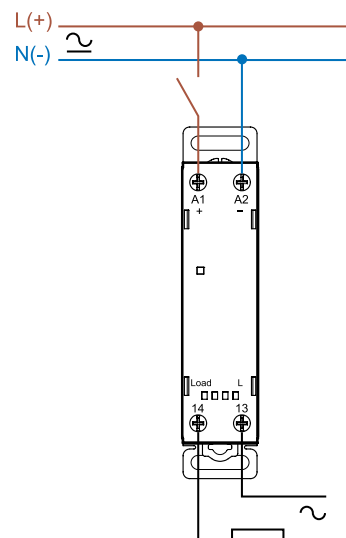
Single-phase connection (77.11/77.21)
