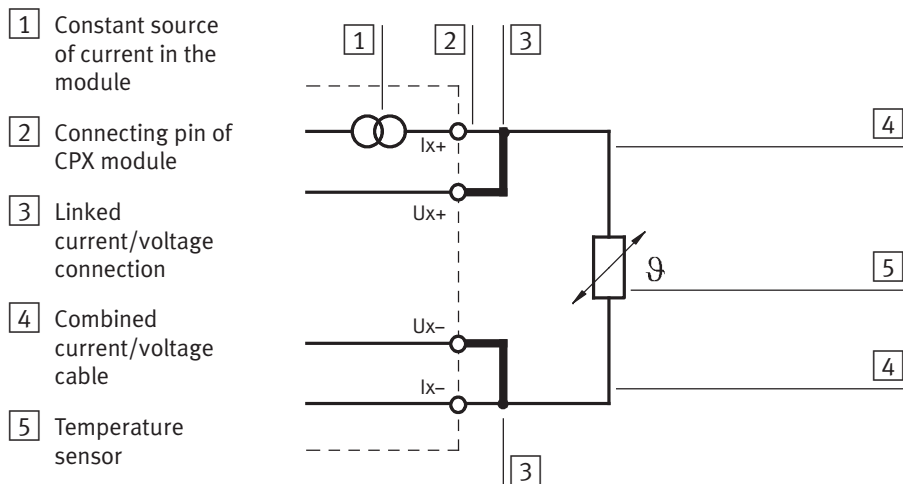
Fig. A/12: Connecting temperature sensors in 2-cable design (CPX-4AE-T)
