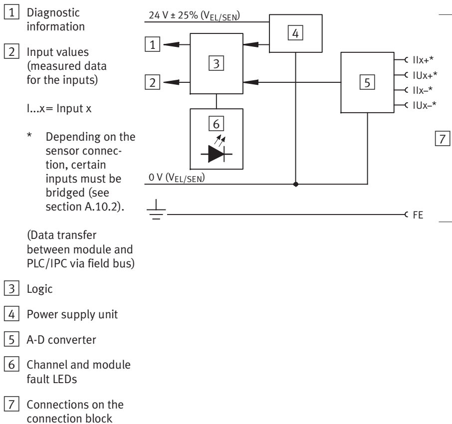
Fig. A/2: Internal structure of CPX-4AE-T
