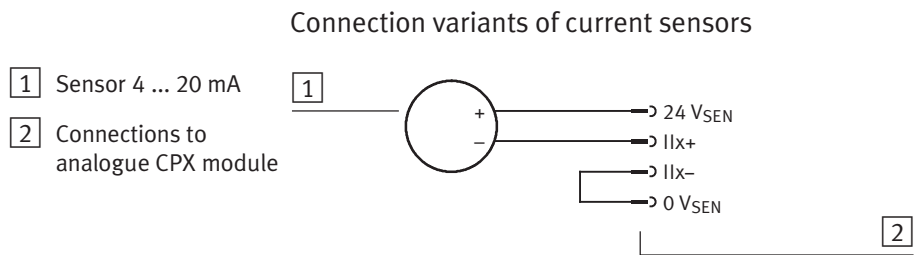
Fig. A/5: Connecting 4 ... 20 mA sensors with internal 24 V power supply (CPX-2AE-U-I, CPX-4AE-I)
