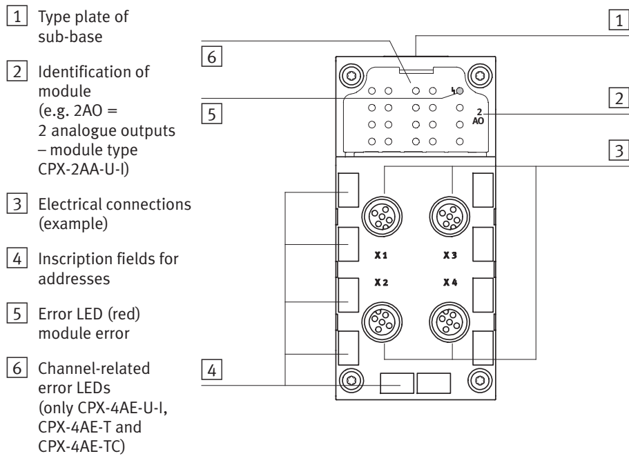
Fig. 1/2: Display and connecting elements
