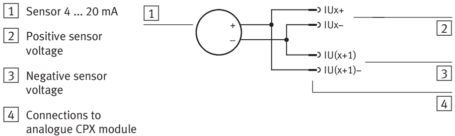
Fig. A/7: Connecting 4 ... 20 mA sensors for reporting of bipolar voltage signals with 2 inputs (CPX-2AE-U-I, CPX-4AE-I)
