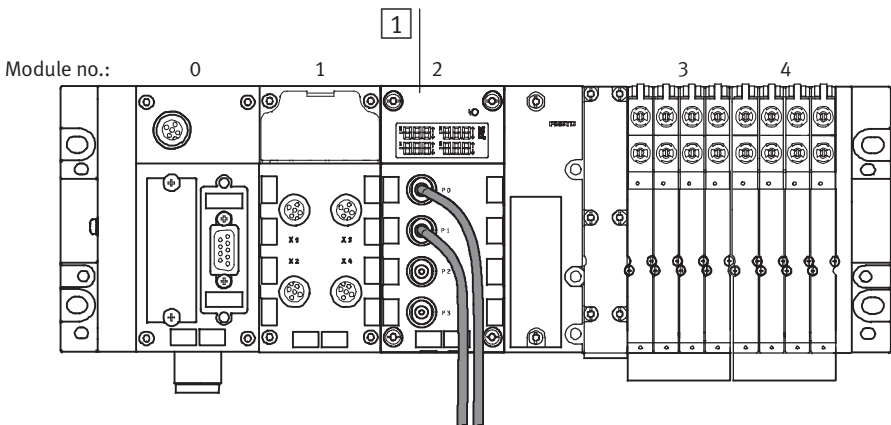
Fig. 7/5: Parameterisation example for pressure sensor module CPX-4AE-P-D10
