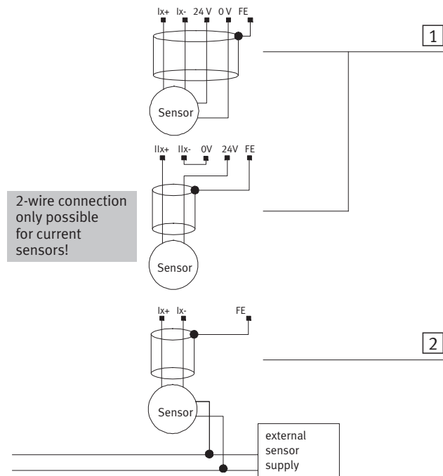
Fig. 3/1: Examples of analogue input connections (screening connection on FE pin)
