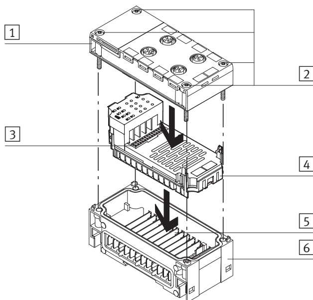
Fig. 1/7: Fitting/removing the I/O module
