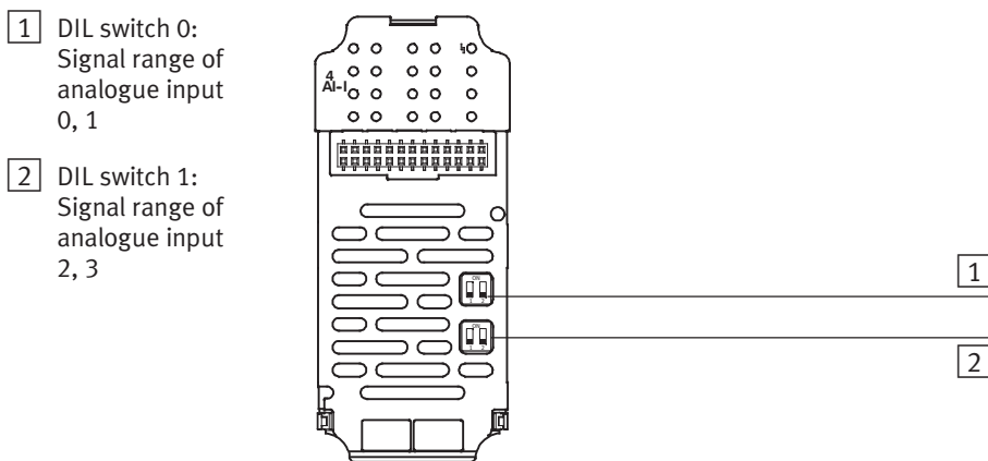
Fig. 4/1: DIL switches in the electronic module (further information on 1 and 2 see following pages)
