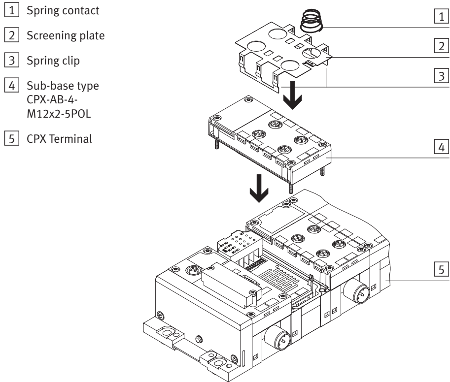
Fig. 1/8: Fitting screening/shield plate type CPX-AB-S-4-12
