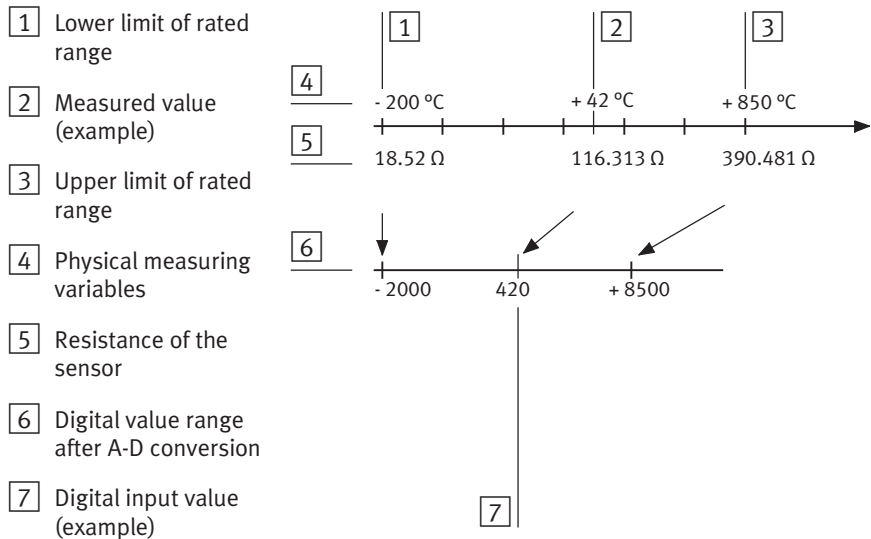
Fig. 5/5: Example: Representing the temperaturesfor a Pt 100 sensor
