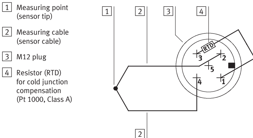
Fig. A/14: Connecting a thermocouple and Pt-1000-RTDs for cold junction compensation by means of an M12 plug to the module CPX-4AE-TC (with connection block CPX-M-4-M12x2-5POL or CPX-AB-4-M12x2-5POL(-R))
