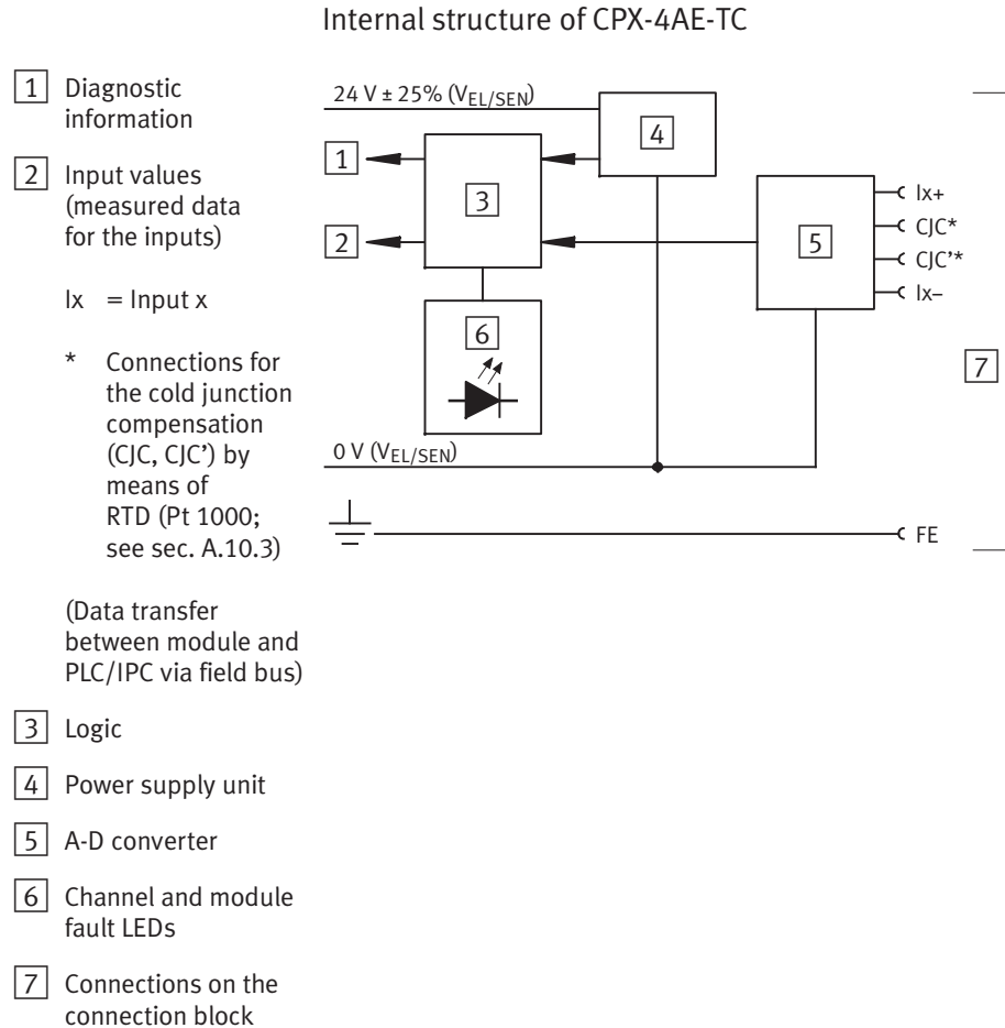
Fig. A/3: Internal structure of CPX-4AE-TC
