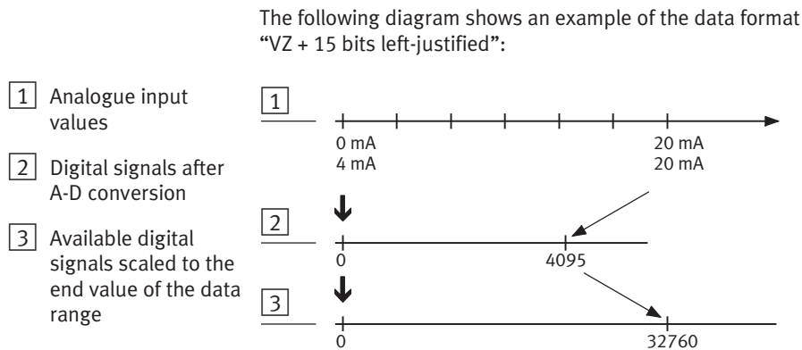
Fig. 4/4: Example of data format “VZ + 15 bits left-justified”
