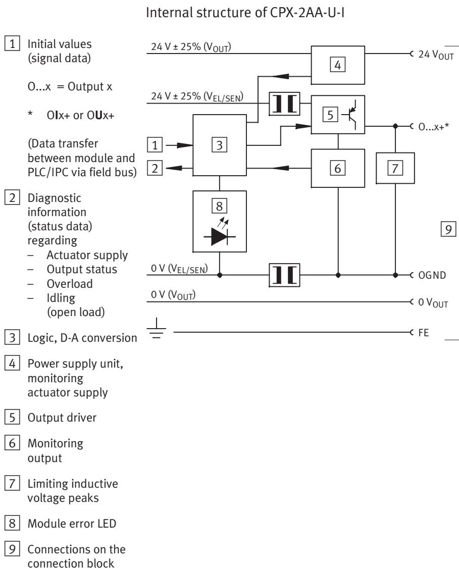
Fig. A/4: Internal structure of CPX-2AA-U-I
