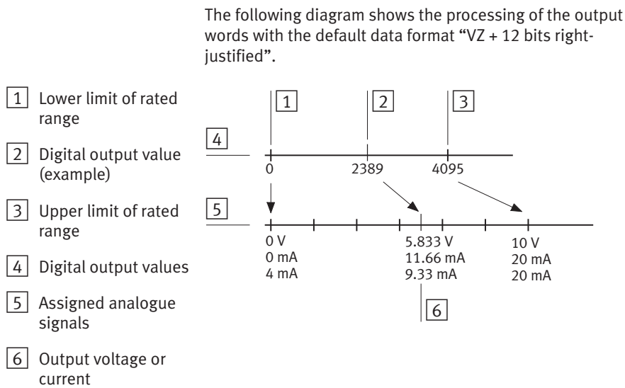
Fig. 8/3: Example of default data format “VZ + 12 bits right-justified”
