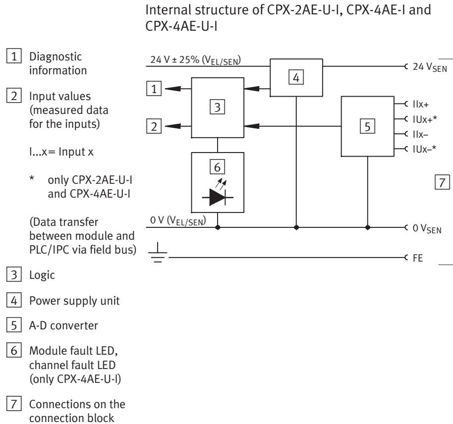
Fig. A/1: Internal structure of CPX-2AE-U-I and CPX-4AE-I
