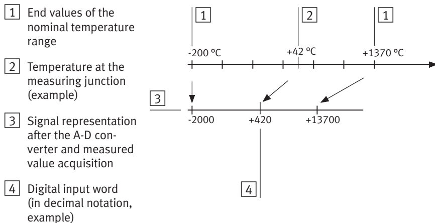
Fig. 6/4: Representation of measured values (example)
