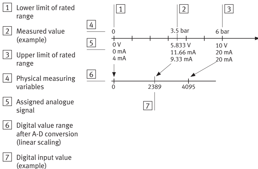
Fig. 2/3: Example of default data format “VZ + 12 bits right-justified”
