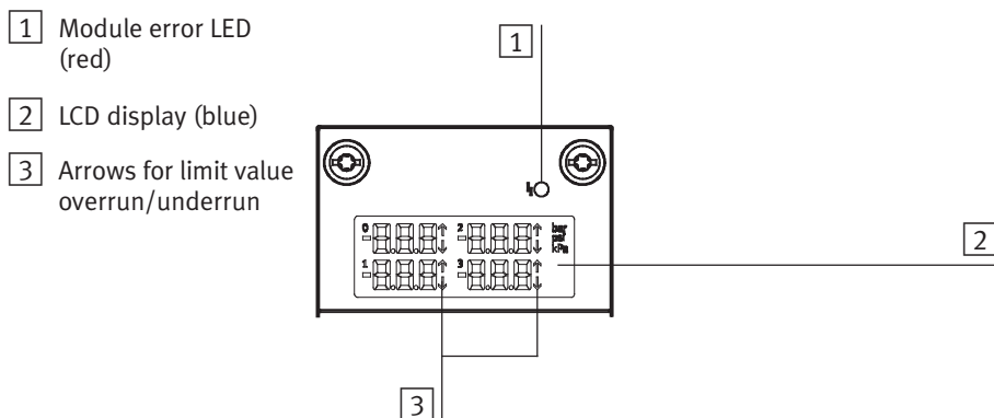
Fig. 7/6: Displays of pressure sensor module CPX-4AE-P
