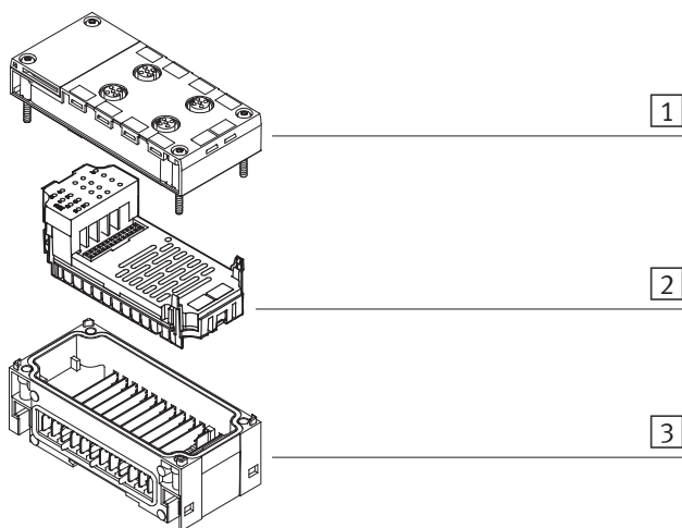
Fig. 1/1: Components of an I/O module
