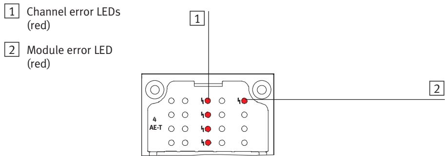
Fig. 5/6: LED displays of the temperature module CPX-4AE-T
