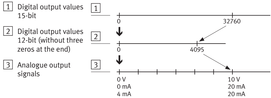
Fig. 8/4: Example of data format “VZ + 15 bits left-justified”
