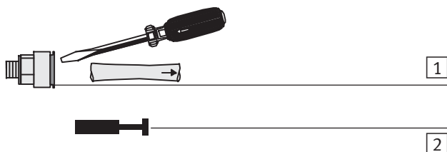
Fig. 7/3: Removing the pneumatic hoses
