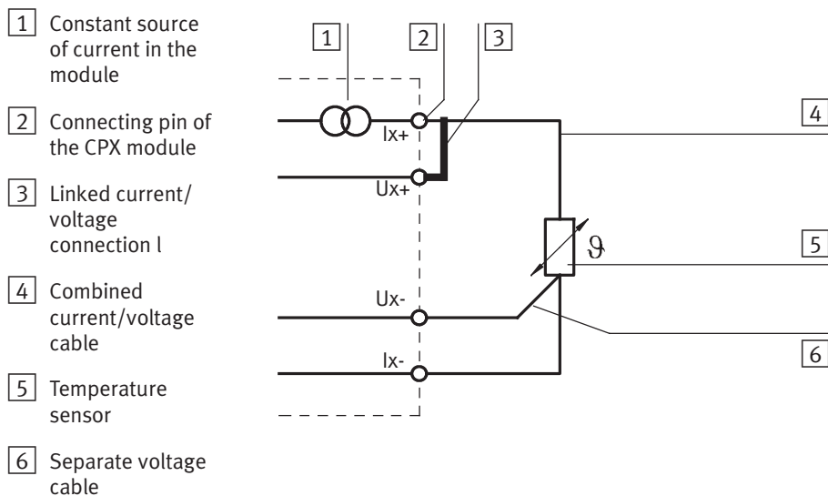
Fig. 5/3: Connection in 3-cable design
