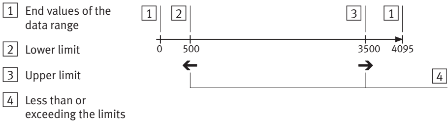
Fig. 2/7: Monitoring of limits with the “Fixed value” data formats
