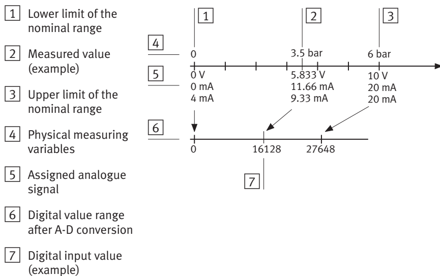
Fig. 3/3: Example data format “VZ + 15 Bit” for a pressure sensor with 0 ... 6 bar and signal ranges 0 ... 10 V, 0 ... 20 mA and 4 ... 20 mA
