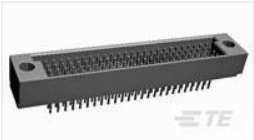
TE Part #532436-3 HDI PIN ASSY 4 ROW 128 POS
