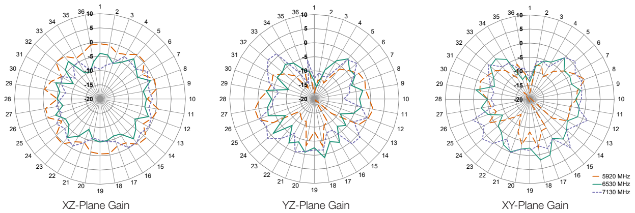
Figure 10. Radiation Patterns for the ANT-W63-WRT Series Antenna at Center of Ground Plane
