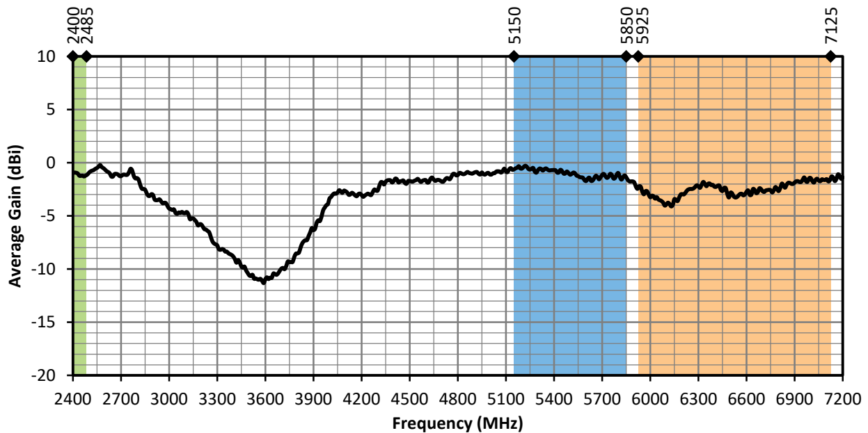
Figure 8. ANT-W63-WRT Antenna Average Gain at Center of Ground Plane
