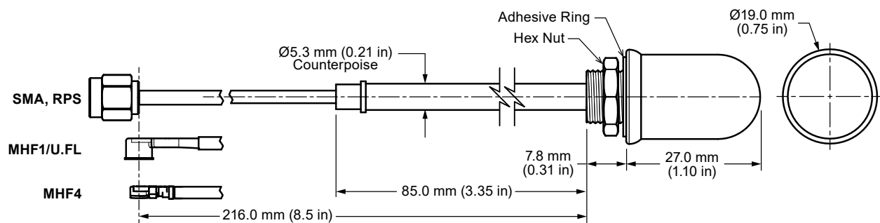
Figure 1. ANT-W63-WRT-ccc Antenna Dimensions
