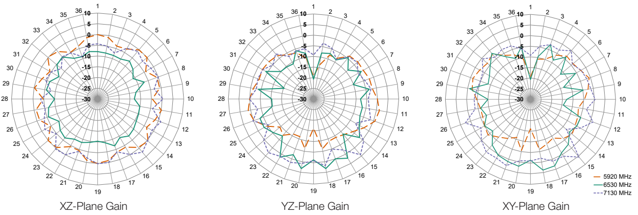
Figure 17. ANT-W63-WRT Antenna Radiation Patterns, Free Space
