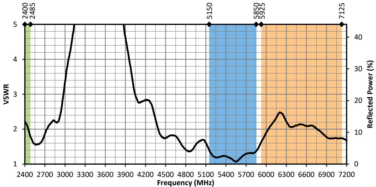
Figure 12. ANT-W63-WRT VSWR, Free Space
