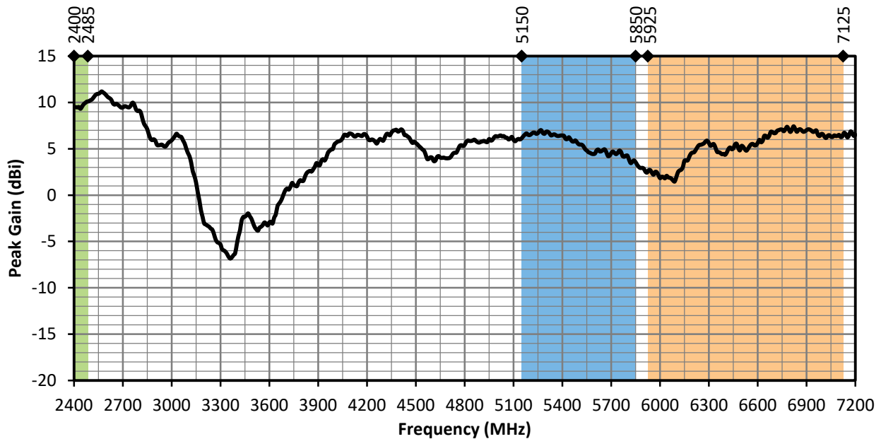
Figure 14. ANT-W63-WRT Peak Gain, Free Space
