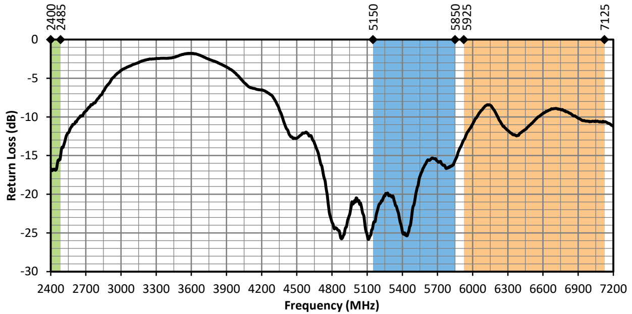
Figure 6. ANT-W63-WRT Antenna Return Loss at Center of Ground Plane
