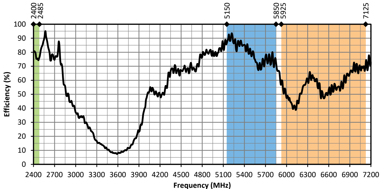
Figure 9. ANT-W63-WRT Antenna Radiation Efficiency at Center of Ground Plane
