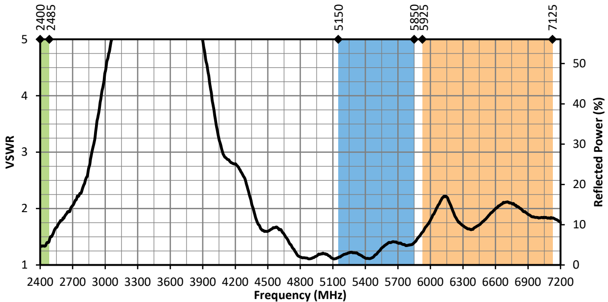
Figure 5. ANT-W63-WRT Antenna VSWR at Center of Ground Plane
