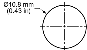
Figure 2. ANT-W63-WRT-ccc Series Antenna Recommended Enclosure Mounting Dimensions
