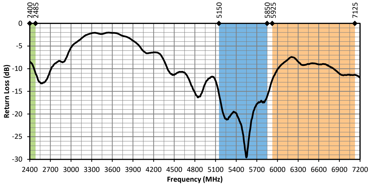
Figure 13. ANT-W63-WRT Return Loss, Free Space
