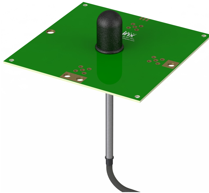
Figure 4. ANT-W63-WRT Series Antenna at Center of Ground Plane
