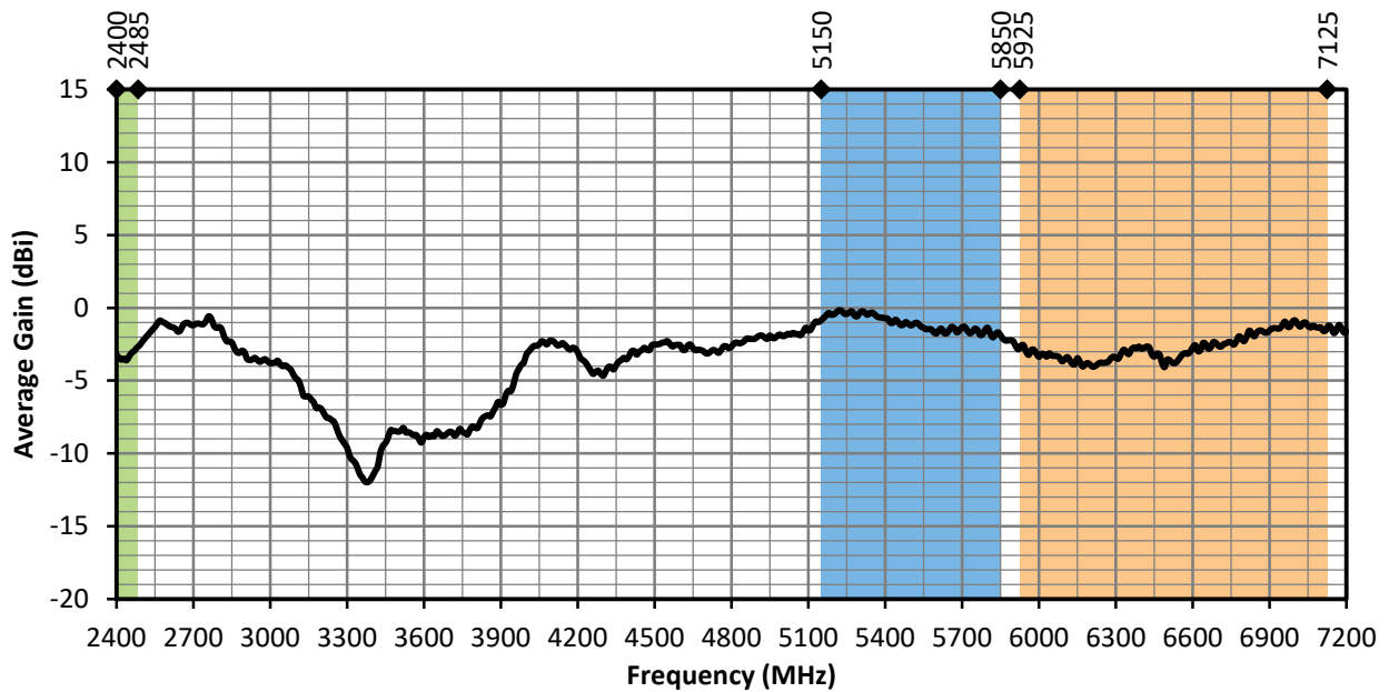
Figure 15. ANT-W63-WRT Antenna Average Gain, Free Space
