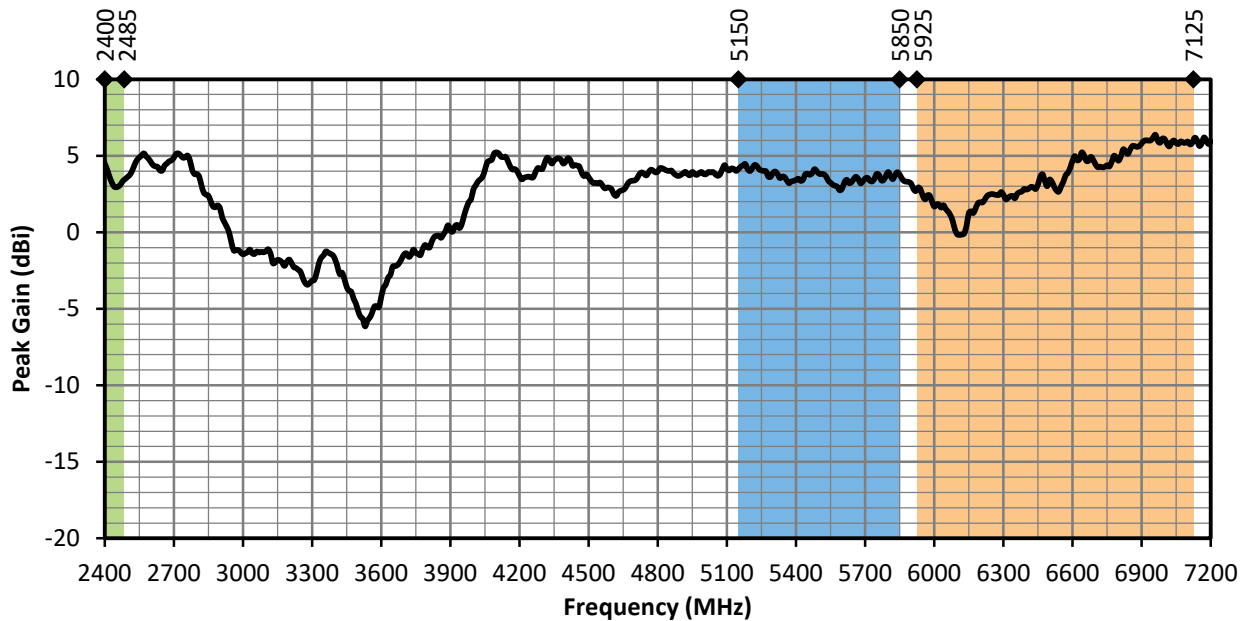
Figure 7. ANT-W63-WRT Antenna Peak Gain at Center of Ground Plane
