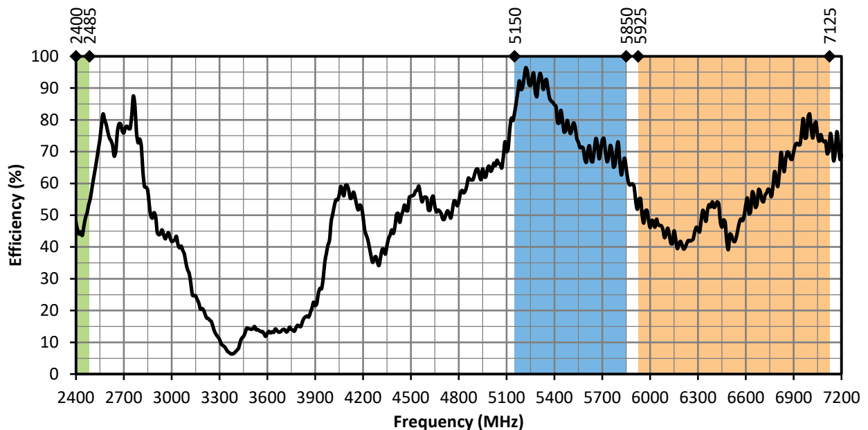
Figure 16. ANT-W63-WRT Series Antenna Radiation Efficiency, Free Space
