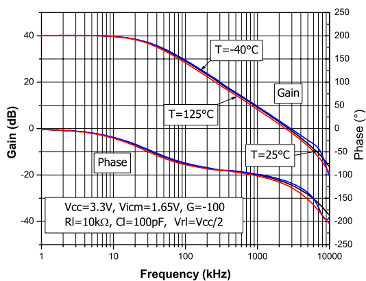
Figure 24. Bode diagram at V_{CC} = 3.3\text{ V}
