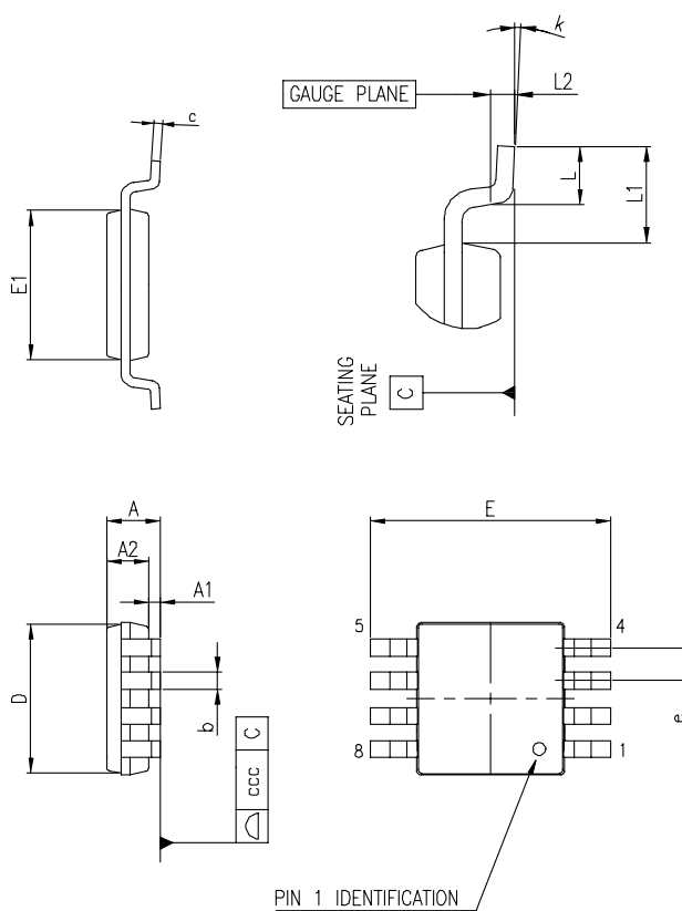
Figure 69. MiniSO8 package outline
