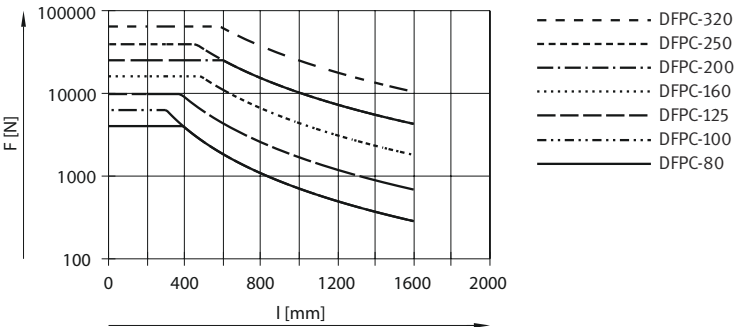
Fig. 3: Permissible buckling load
