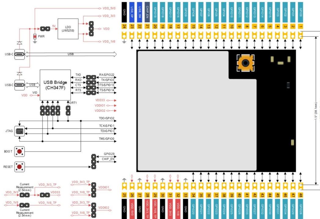
Figure 3: MQM748 Module Development Kit Block Diagram
