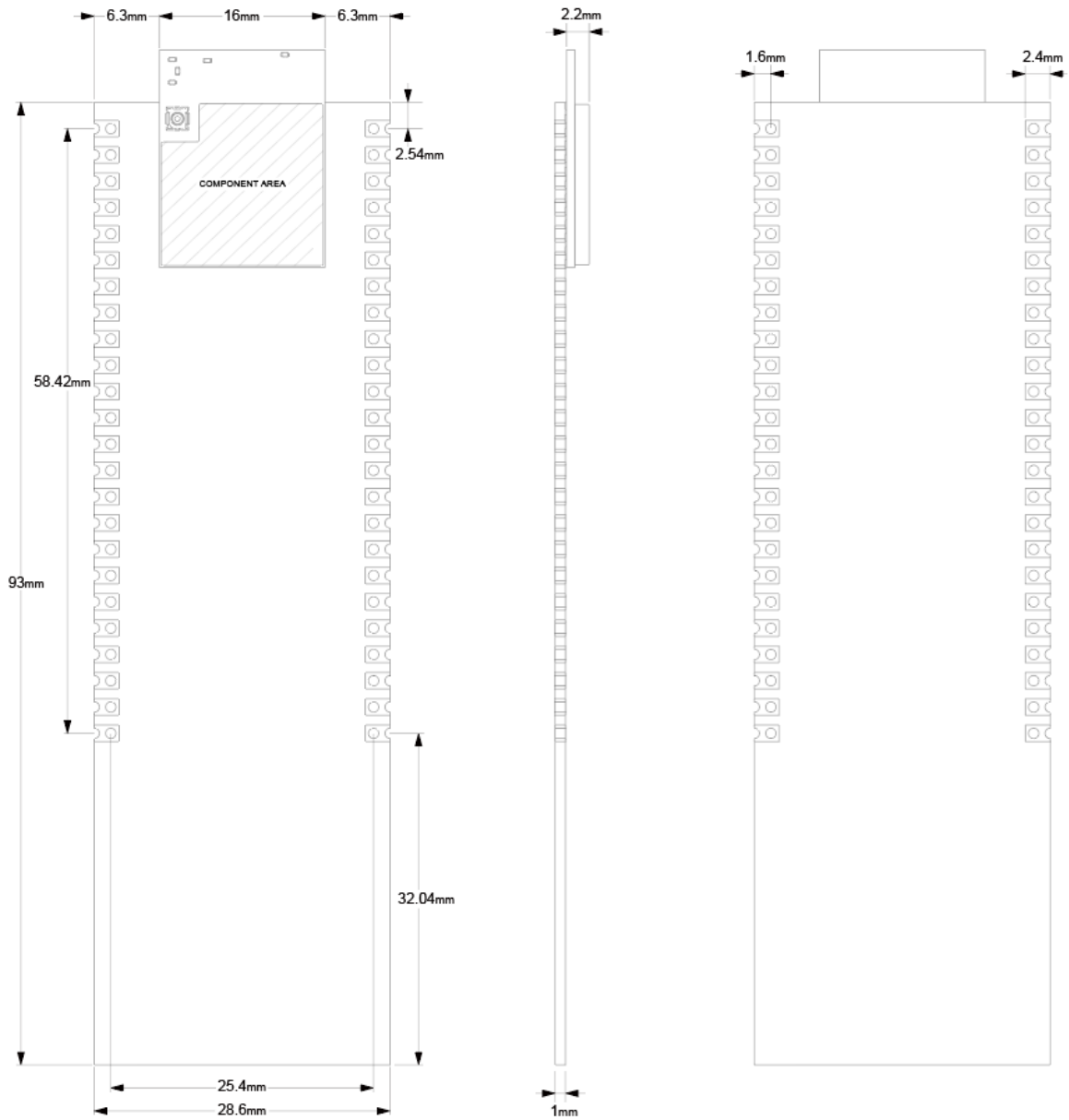
Figure 5: MQM748 Module Development Kit Dimension
