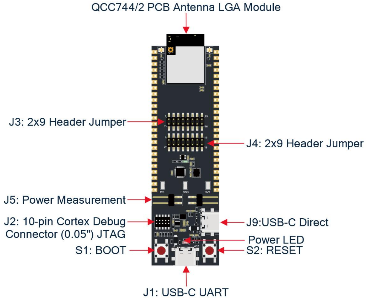
Figure 4: MQM748 Module Development Kit Component Layout
