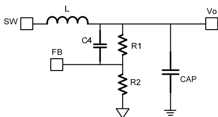
Figure 8: Simplified Circuit without External Ramp
