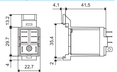
056.27 with relay
