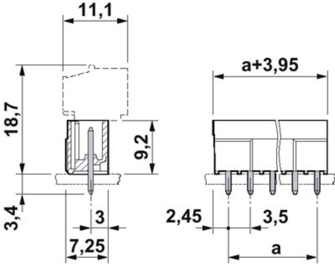
Dimensioned drawing
