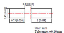
Recommended Soldering Pad Dimensions
