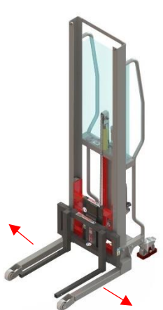
855 000 966 - Sliding forks
