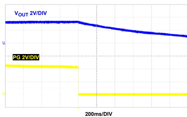
FIGURE 48. OVER-TEMPERATURE PROTECTION
