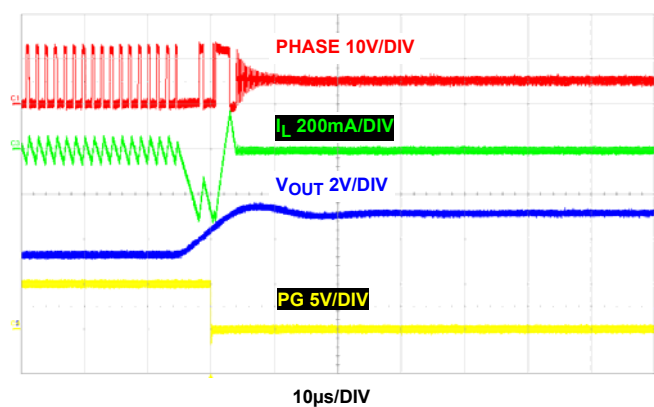
FIGURE 47. OVERVOLTAGE PROTECTION
