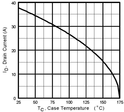
Fig 9. Maximum Drain Current Vs. Case Temperature
