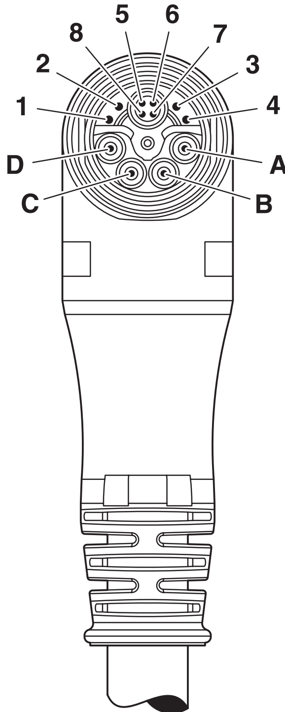
Schematic diagram
