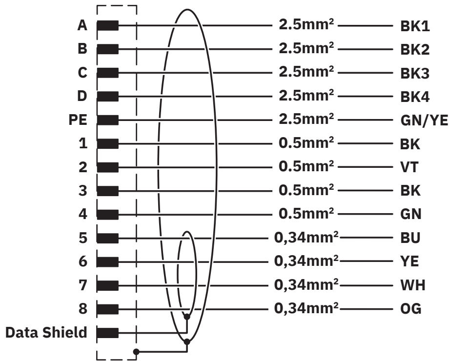
Circuit diagram
