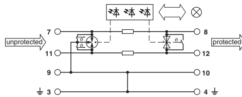
Application drawing
