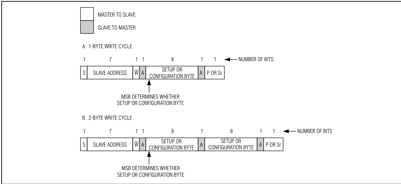
Figure 9. Write Cycle
