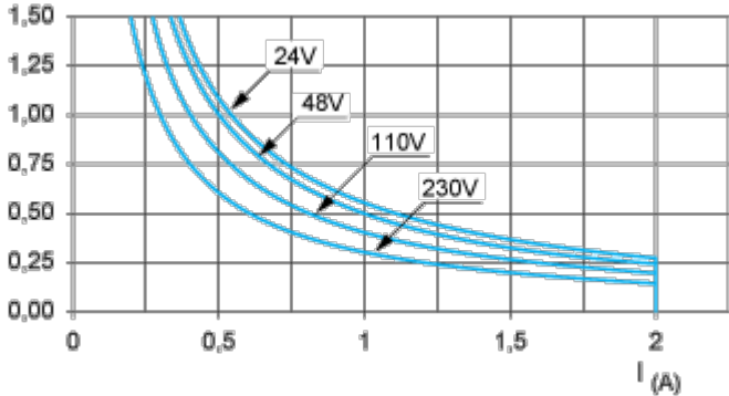
Courbes AC12
