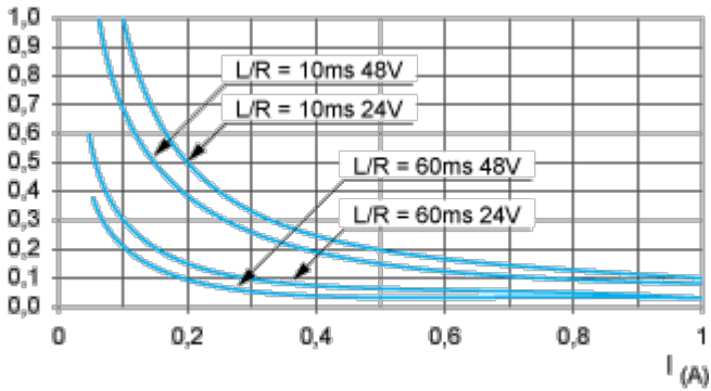
Courbes DC13
