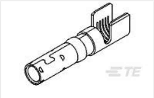
TE Part #213847-3 POWERBAND CONT ASSY,SILVER PLT
