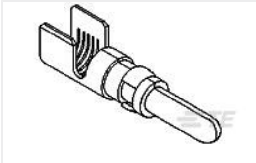
TE Part #213845-3 POWERBAND CONT ASSY,SILVER PLT
