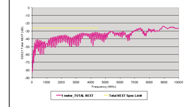
Total NEXT of 4x Mini-SAS unequalized 1 meter cable assembly
