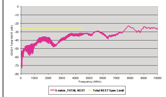
Total NEXT of 4x Mini-SAS equalized 5 meter cable assembly
