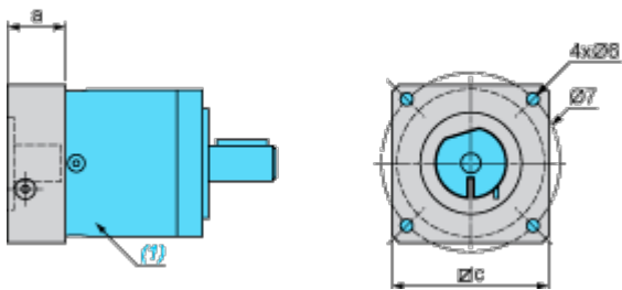
(1) Gearbox
