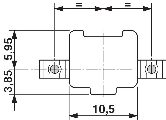
Dimensional drawing
