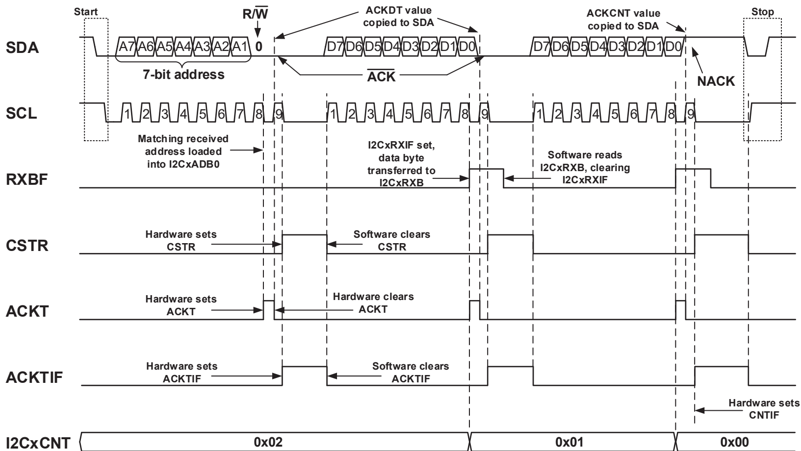
Figure 39-15. 7-Bit Client Mode Transmission (ACKTIE = 1)
