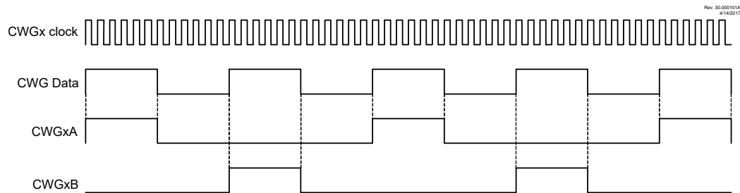
Figure 34-10. Example of Synchronous Steering ( MODE = 'b001)
