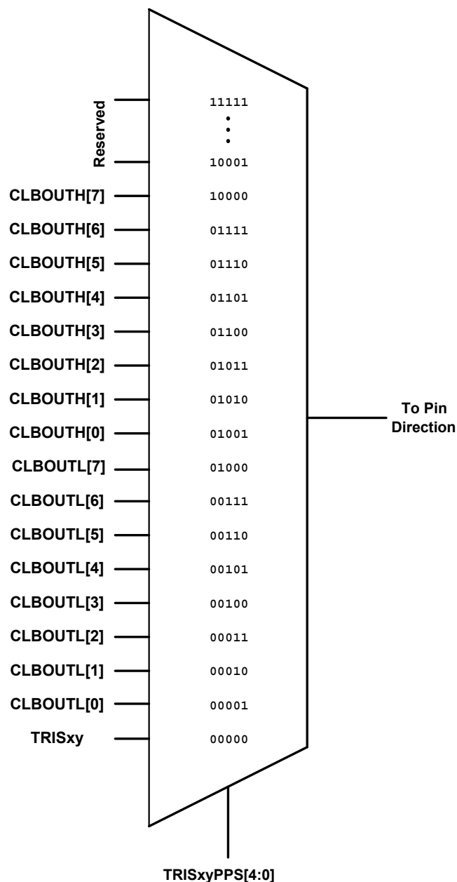
Figure 25-8. TRISxyPPS Output Selections
