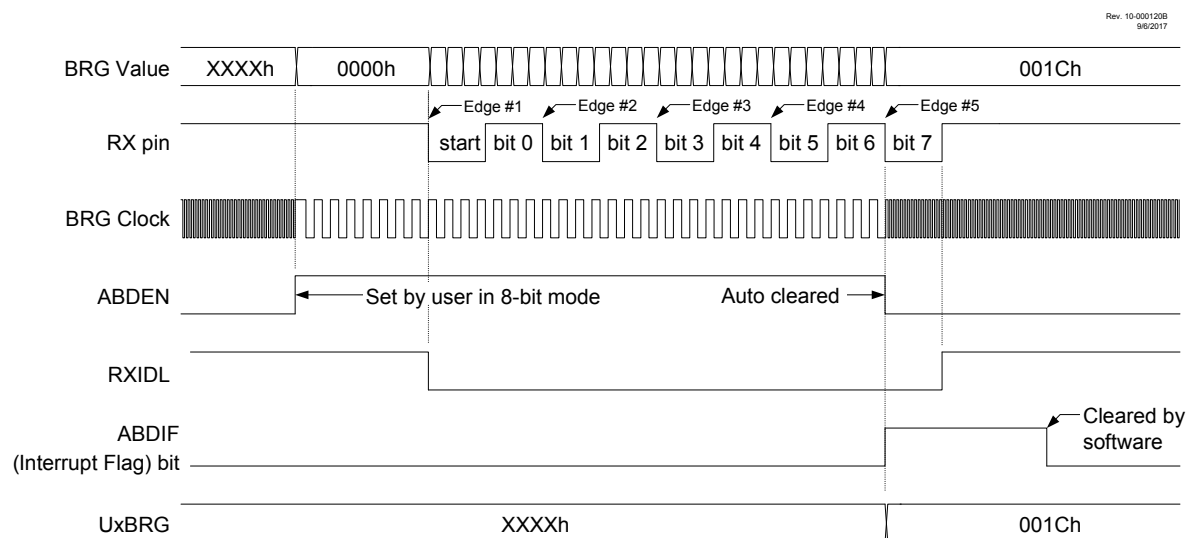
Figure 37-12. Automatic Baud Rate Calibration
