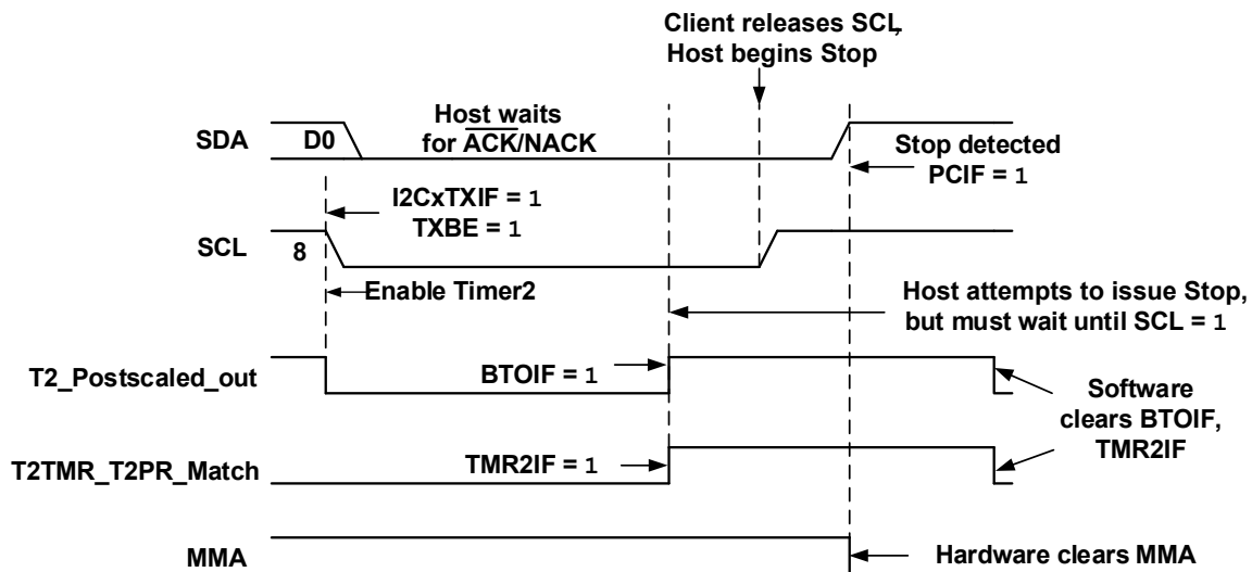
Figure 39-8. Host Mode Bus Time-Out Example
