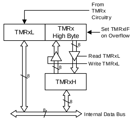
Figure 28-3. Timer1 16-Bit Read/Write Mode Block Diagram
