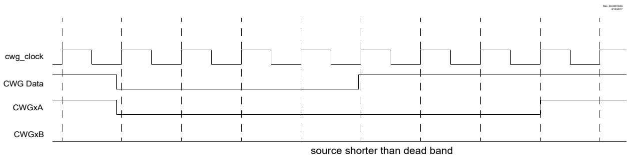
Figure 34-13. Dead-Band Operation, CWGxDBR = 0 \times 03 , CWGxDBF = 0 \times 06 , Source Shorter Than Dead Band
