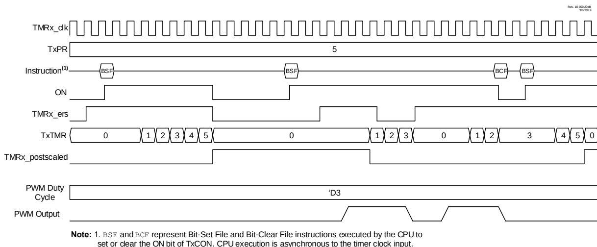
Figure 29-12. Level Triggered Hardware Limit One Shot Mode Timing Diagram (MODE = 'b10110)
