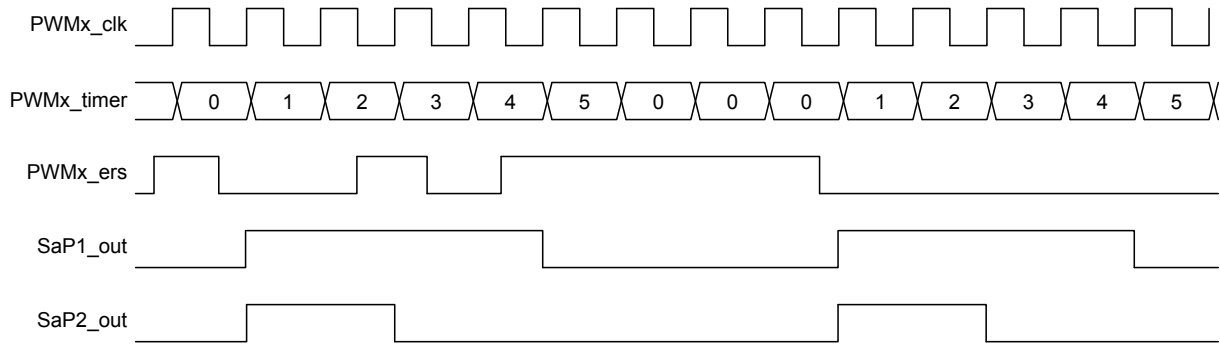
Figure 33-16. Left Aligned Mode with ERSNOW = 0
