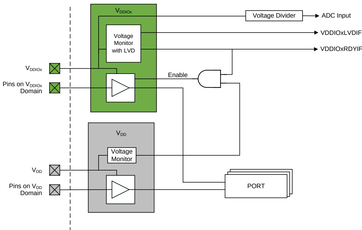
Figure 23-1. POR and Voltage Monitors on MVIO Domain
