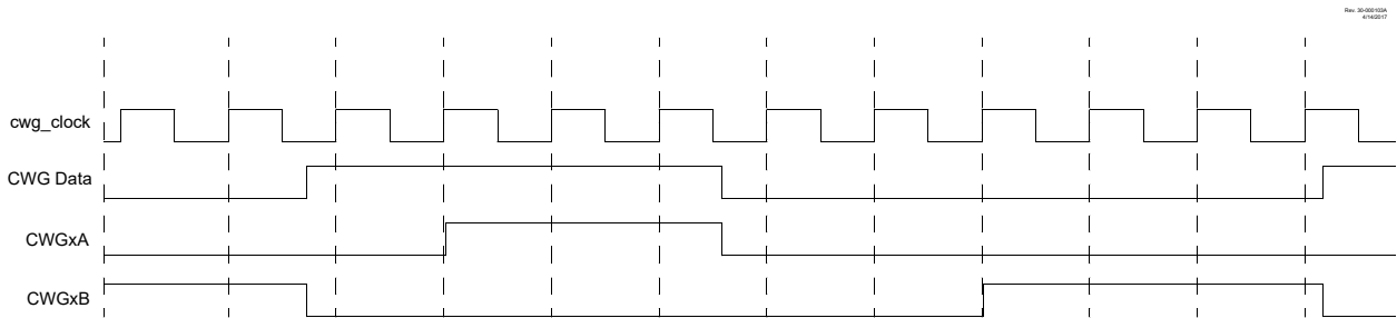
Figure 34-12. Dead-Band Operation, CWGxDBR = 0 \times 01 , CWGxDBF = 0 \times 02
