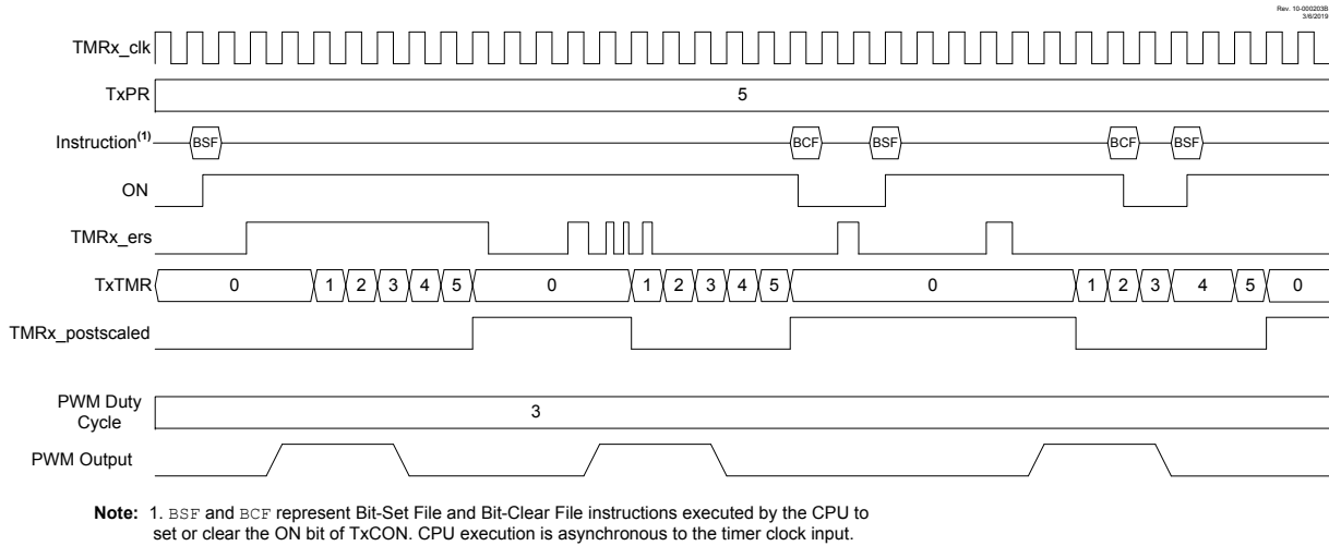
Figure 29-11. Rising Edge Triggered Monostable Mode Timing Diagram (MODE = 'b10001)
