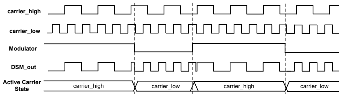
Figure 36-6. Full Synchronization (MDCHSYNC = 1, MDCLSYNC = 1)
