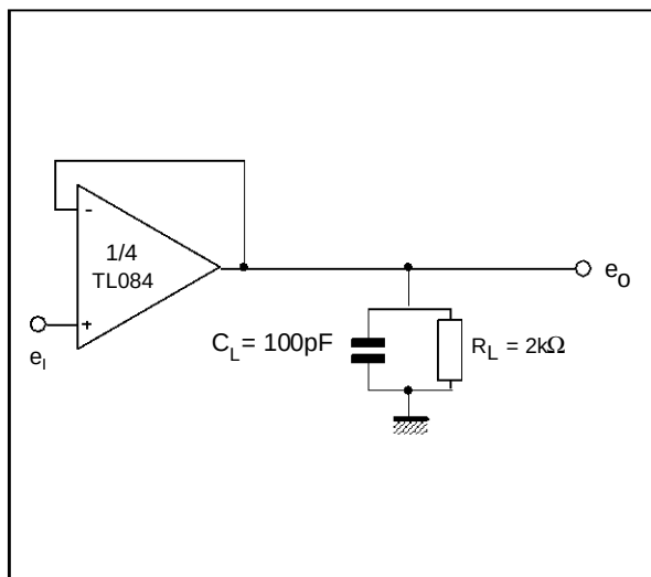
Figure 1 : Voltage Follower
