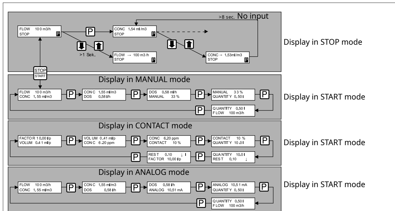
Fig. 16: Overview of continuous displays
