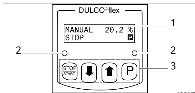
Fig. 13: Control unit
