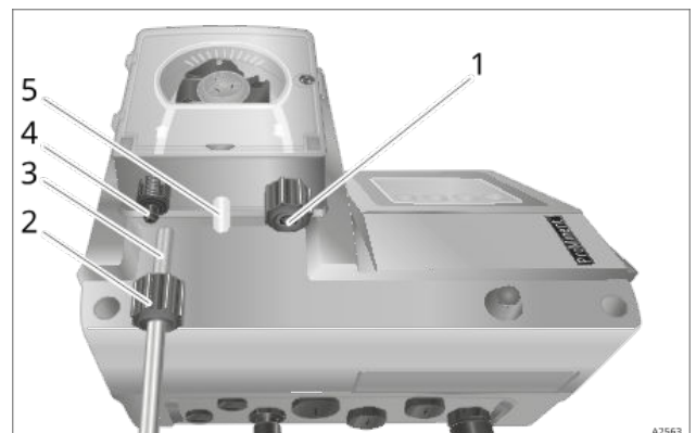
Fig. 9: Assembling the suction and metering line
