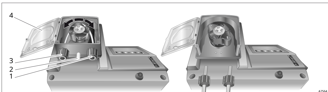
Fig. 21: Replacing the pump hose
