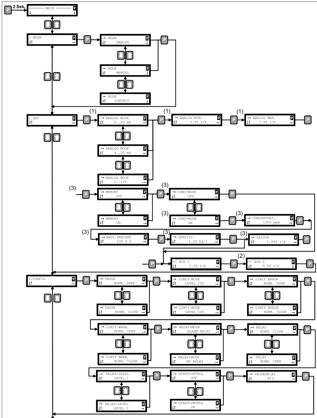
Fig. 18: Overview of DF4a operating menu
