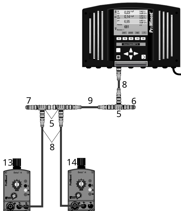
Fig. 24: CAN connector for metering pumps
