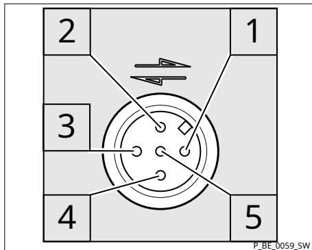
Fig. 25: Pump pin assignment (male)
