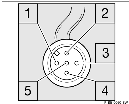
Fig. 26: Pump pin assignment (female)
