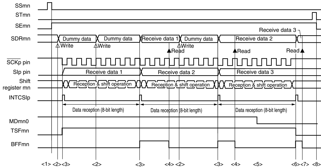
&lt;R&gt; Figure 13-38. Timing Chart of Master Reception (in Continuous Reception Mode) (Type 1: DAPmn = 0, CKPmn = 0)
