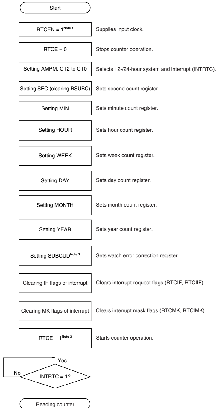
Figure 8-19. Procedure for Starting Operation of Real-Time Counter
