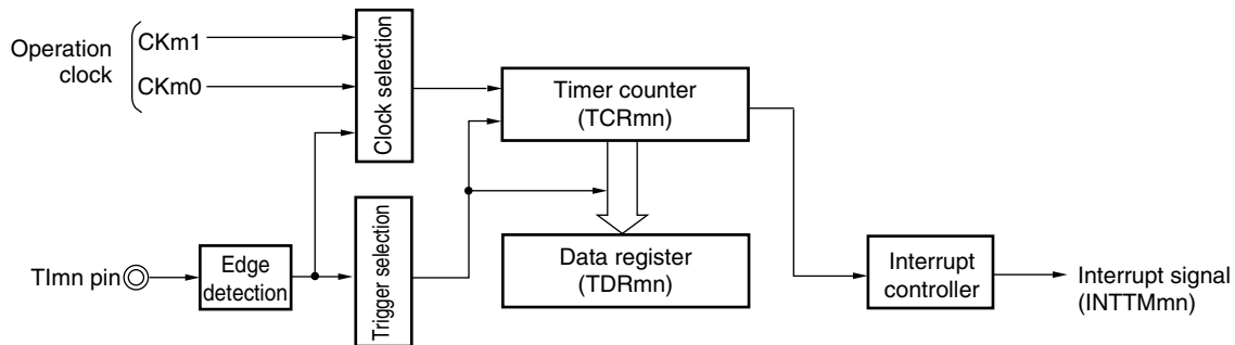
Figure 7-53. Block Diagram of Operation as Input Signal High-/Low-Level Width Measurement
