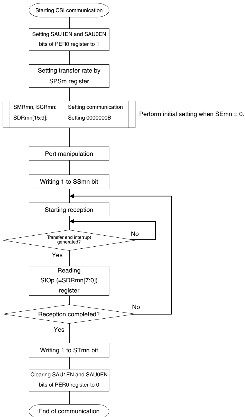
Figure 13-61. Flowchart of Slave Reception (in Single-Reception Mode)
