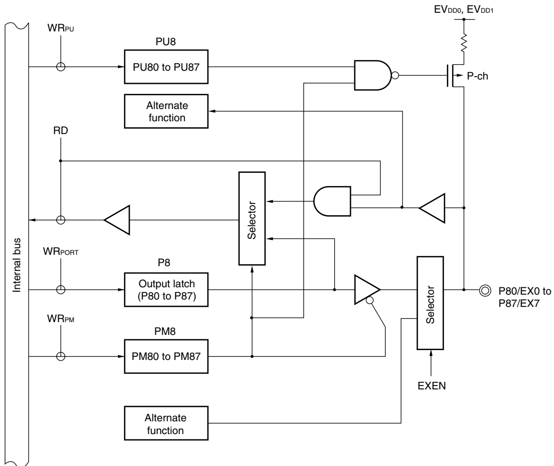
Figure 4-31. Block Diagram of P80 to P87
