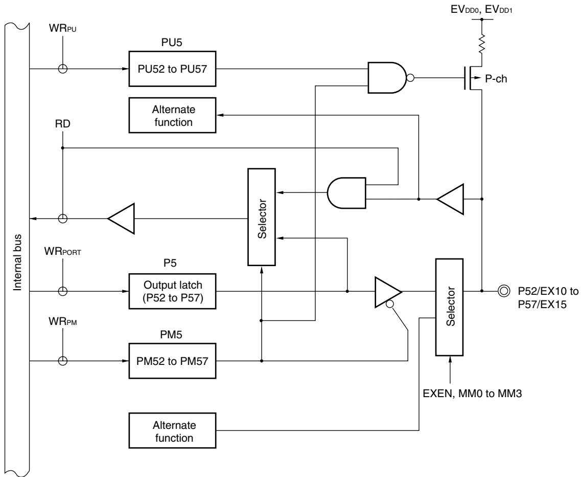
Figure 4-26. Block Diagram of P52 to P57
