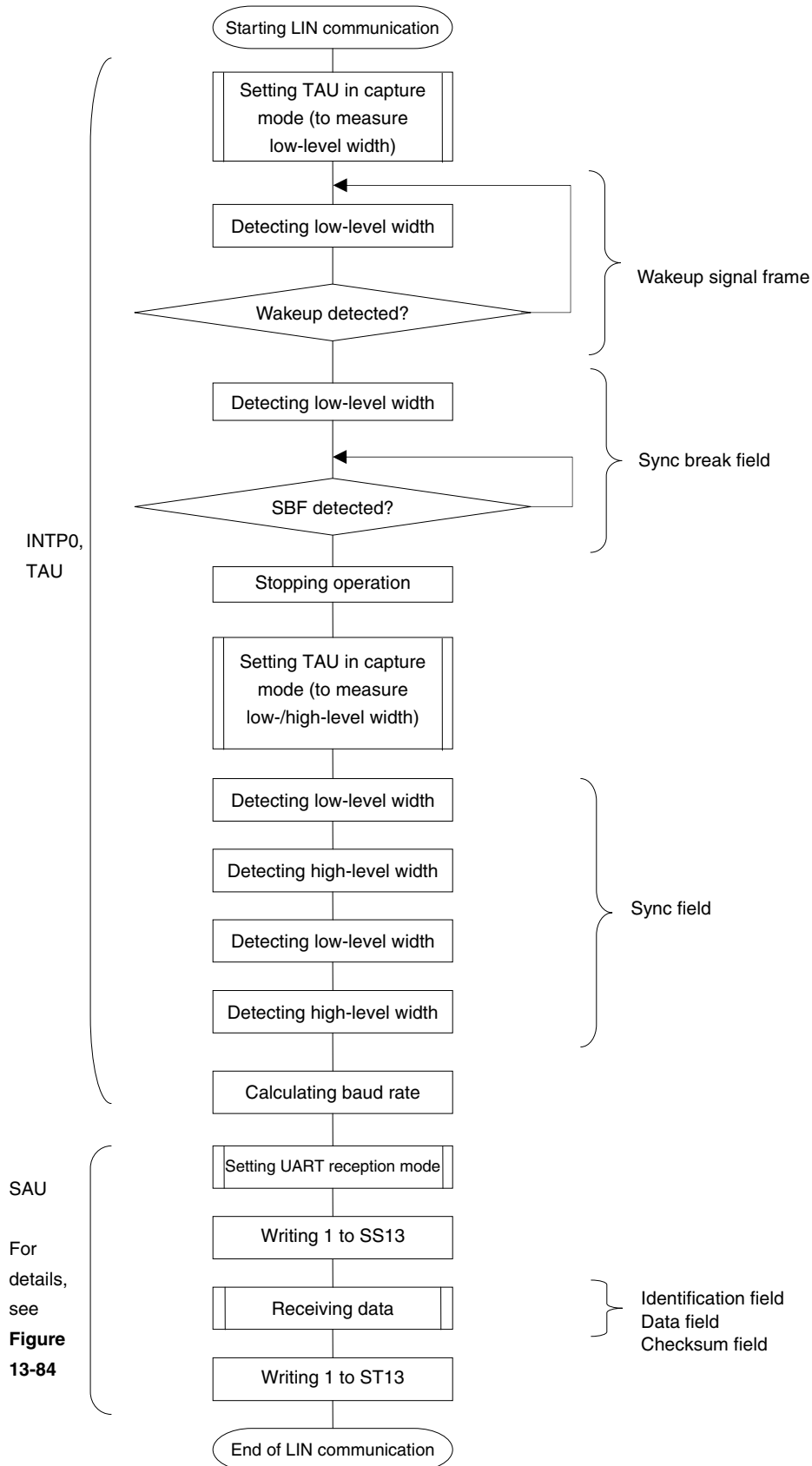
Figure 13-89. Flowchart of LIN Reception
