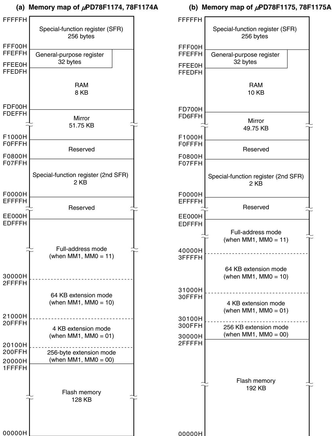
Figure 5-1. Memory Map When Using External Bus Interface Function (1/3)
