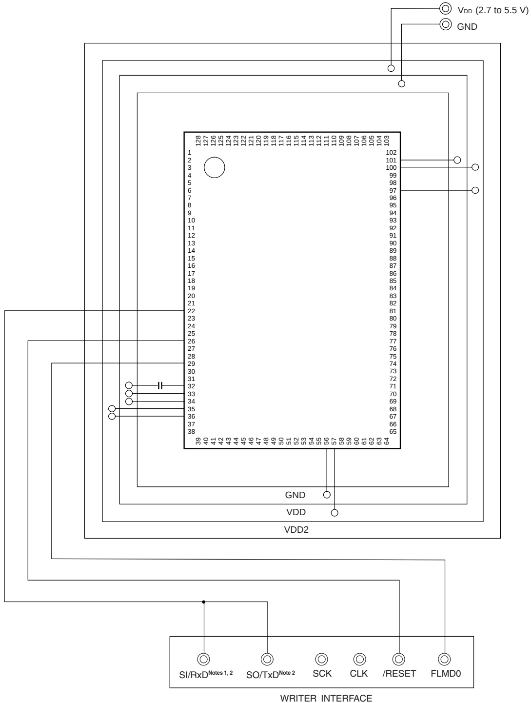
Figure 25-1. Example of Wiring Adapter for Flash Memory Writing
