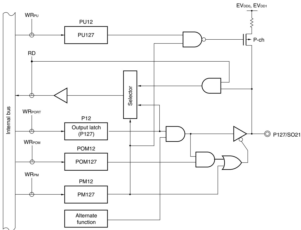
Figure 4-42. Block Diagram of P127
