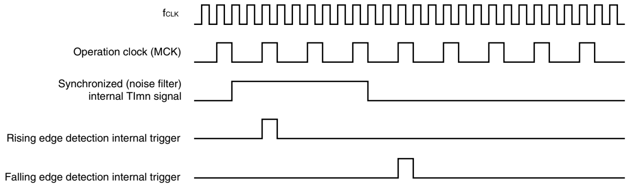
Figure 7-36. Edge Detection Basic Operation Timing
