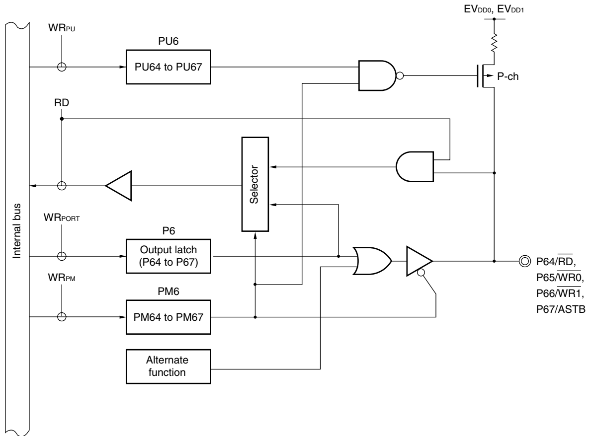
Figure 4-29. Block Diagram of P64 to P67
