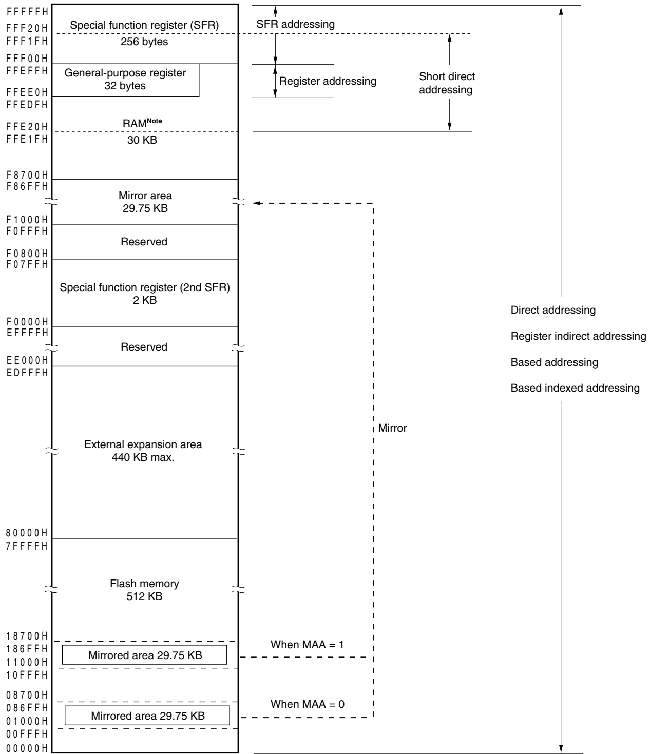
<R> Figure 3-11. Correspondence Between Data Memory and Addressing ( \mu PD78F1178, 78F1178A)
