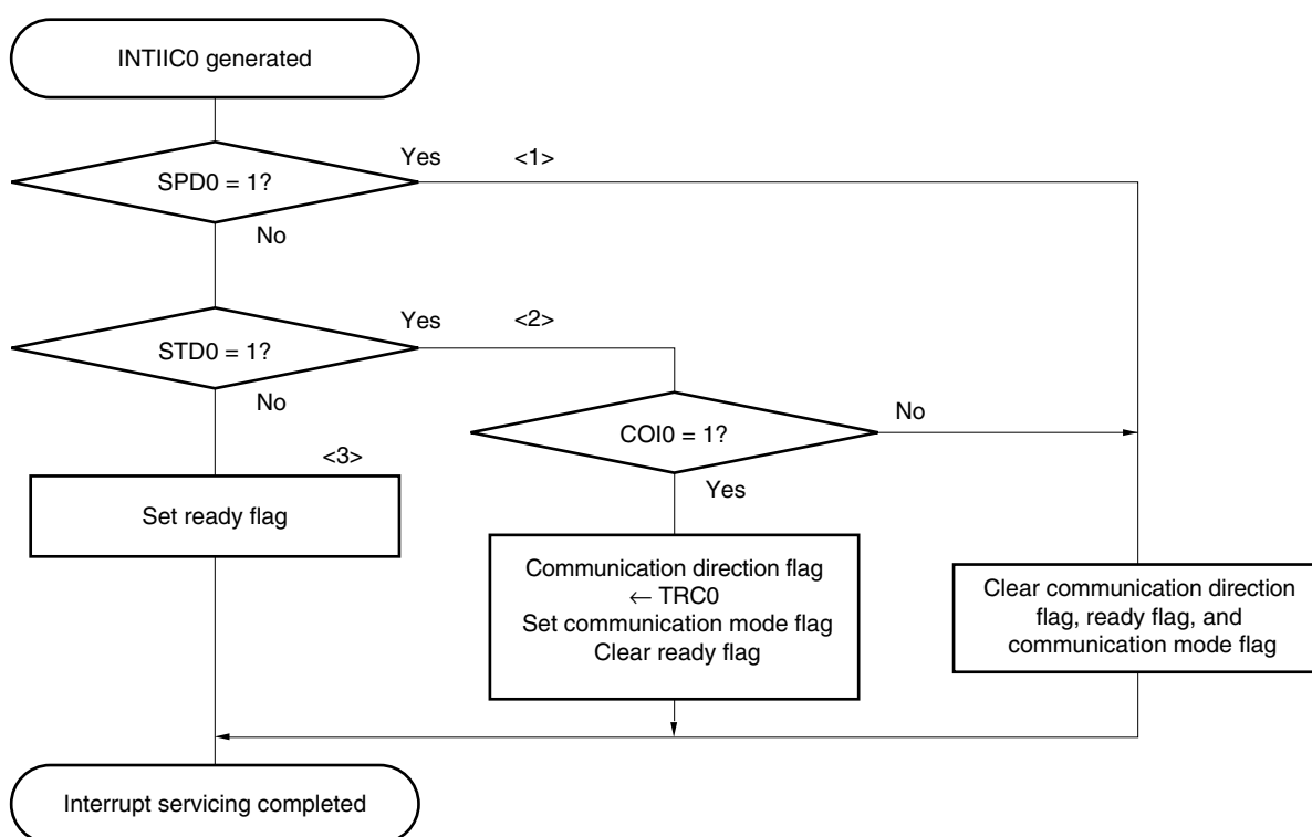
Figure 14-27. Slave Operation Flowchart (2)
