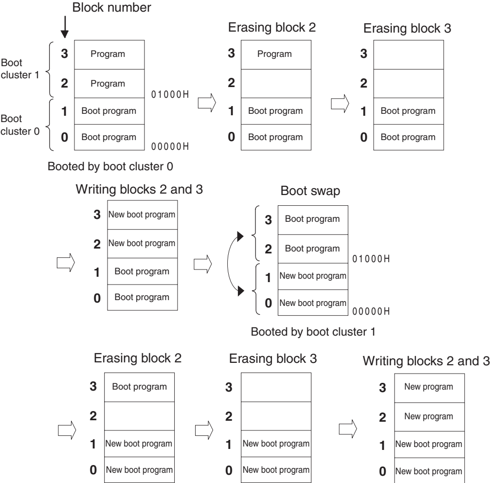
Figure 25-12. Example of Executing Boot Swapping
