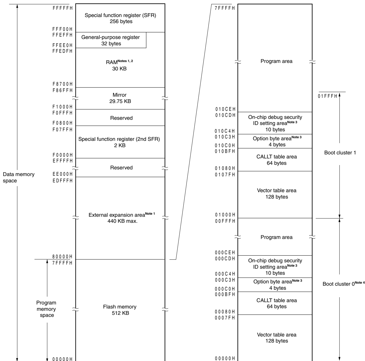
Figure 3-5. Memory Map (μPD78F1178, 78F1178A)
