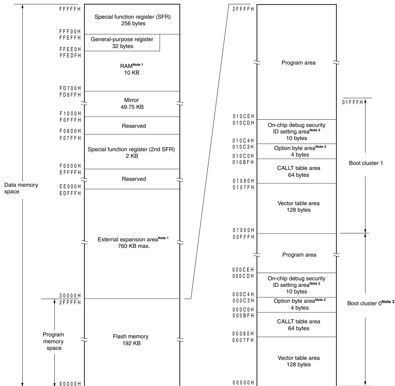
Figure 3-2. Memory Map ( \mu PD78F1175, 78F1175A)
