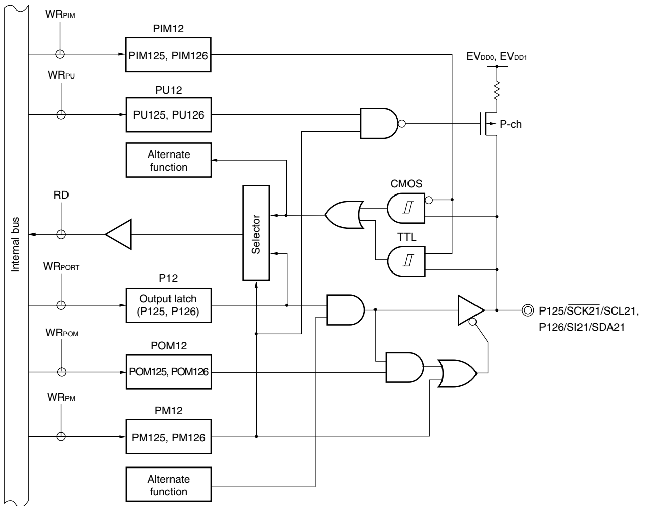
Figure 4-41. Block Diagram of P125 and P126
