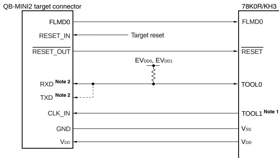
Figure 26-1. Connection Example of QB-MINI2 and 78K0R/KH3
