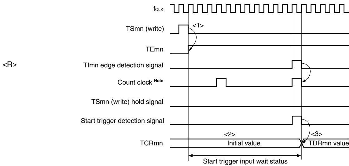
Figure 7-14. Start Timing (In One-count Mode)
