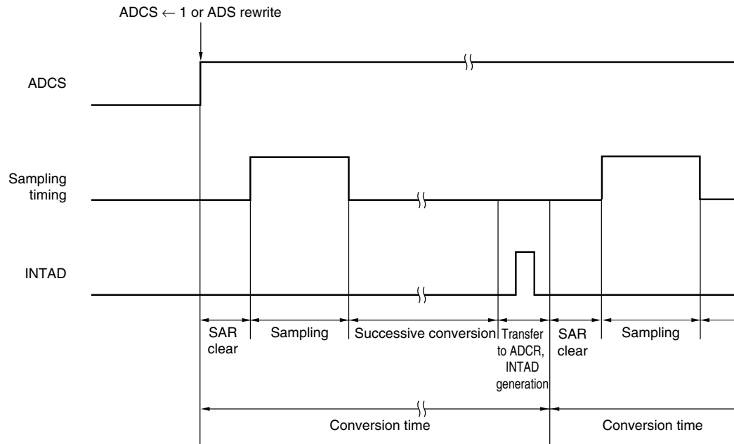
Figure 11-6. A/D Converter Sampling and A/D Conversion Timing
