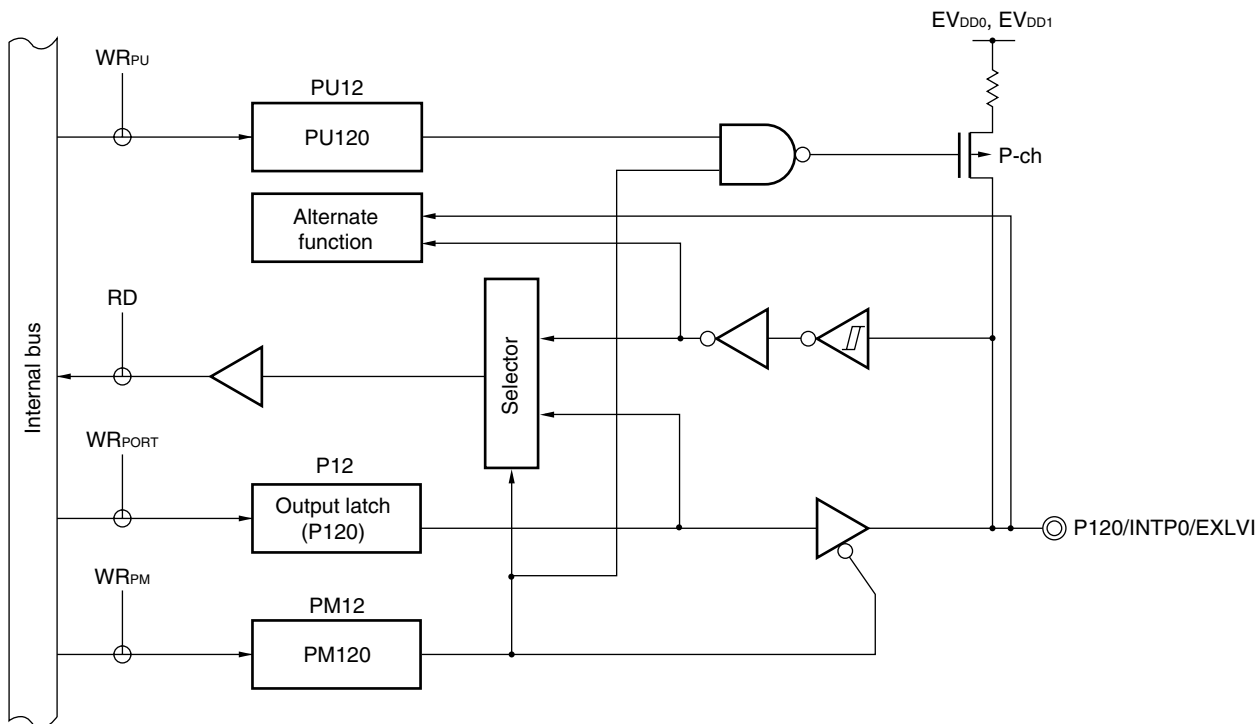
Figure 4-38. Block Diagram of P120
