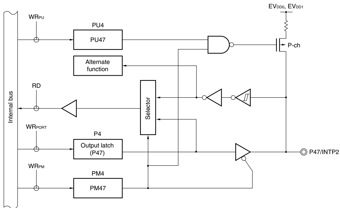
Figure 4-24. Block Diagram of P47
