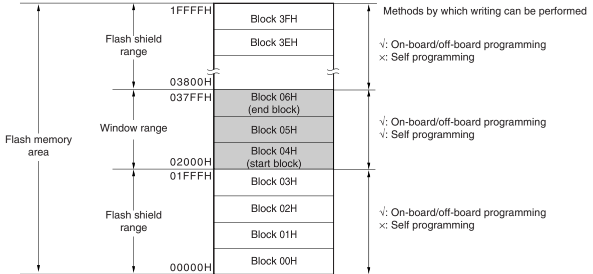
Figure 25-13. Flash Shield Window Setting Example (Target Devices: \mu PD78F1174, 78F1174A, Start Block: 04H, End Block: 06H)
