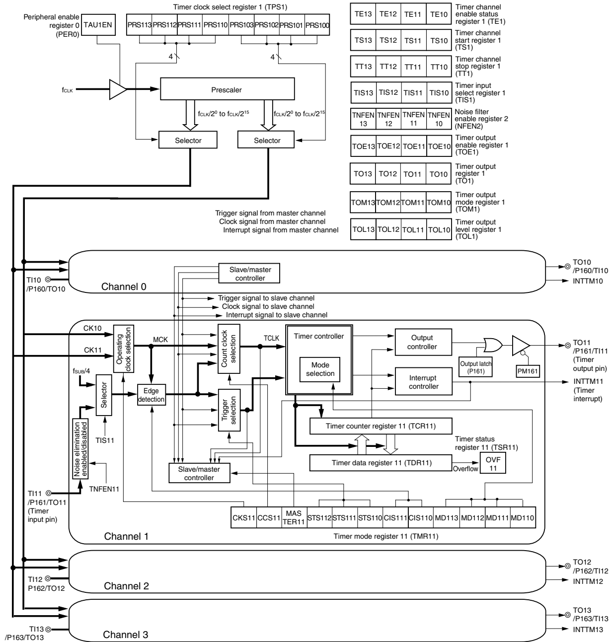
Figure 7-2. Block Diagram of Timer Array Unit 1
