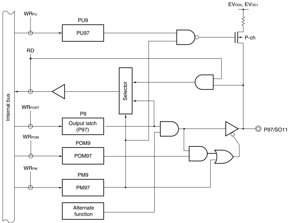
Figure 4-35. Block Diagram of P97
