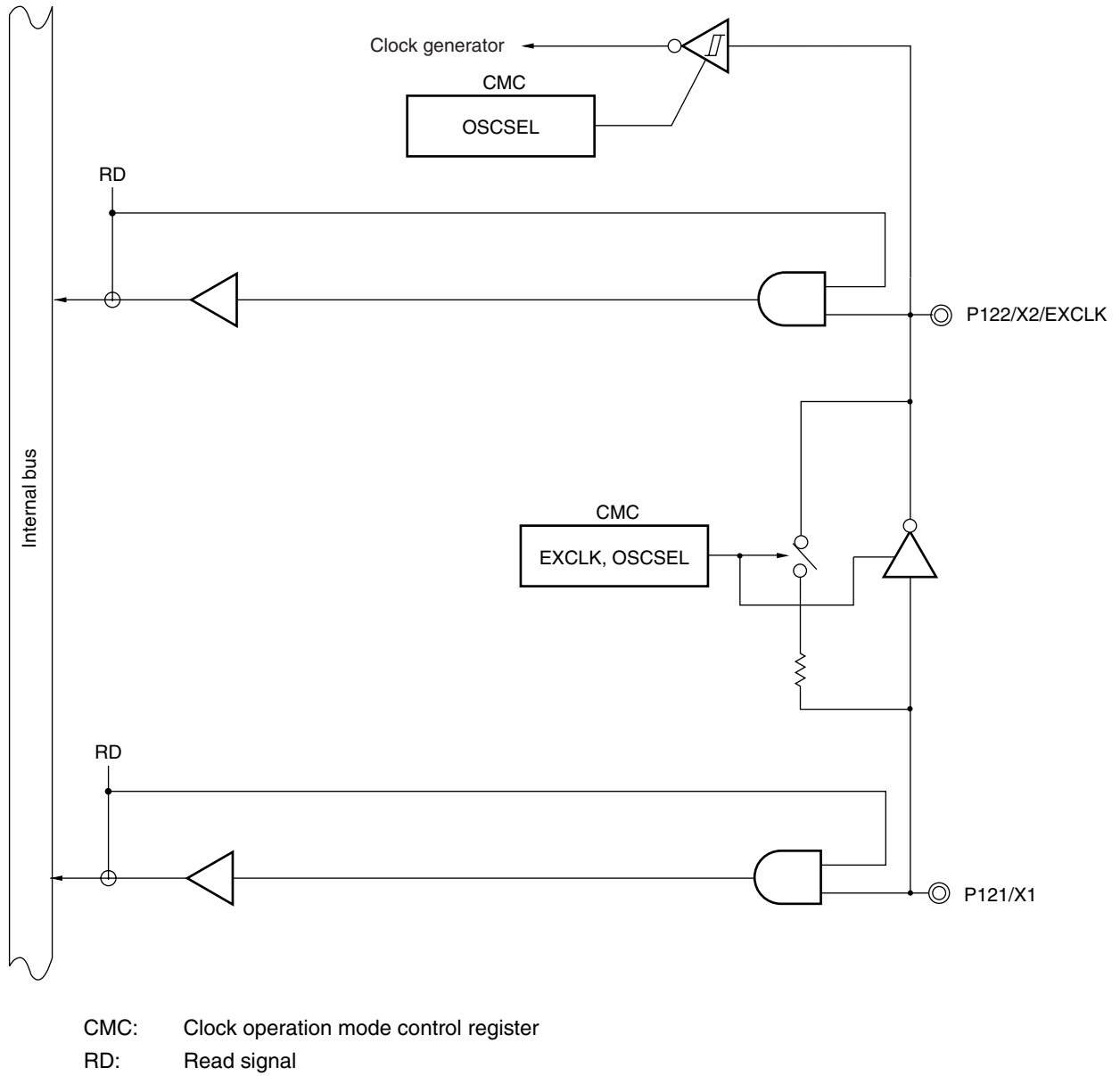
Figure 4-39. Block Diagram of P121 and P122
