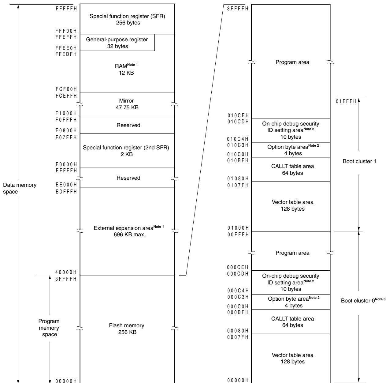
Figure 3-3. Memory Map ( \mu PD78F1176, 78F1176A)
