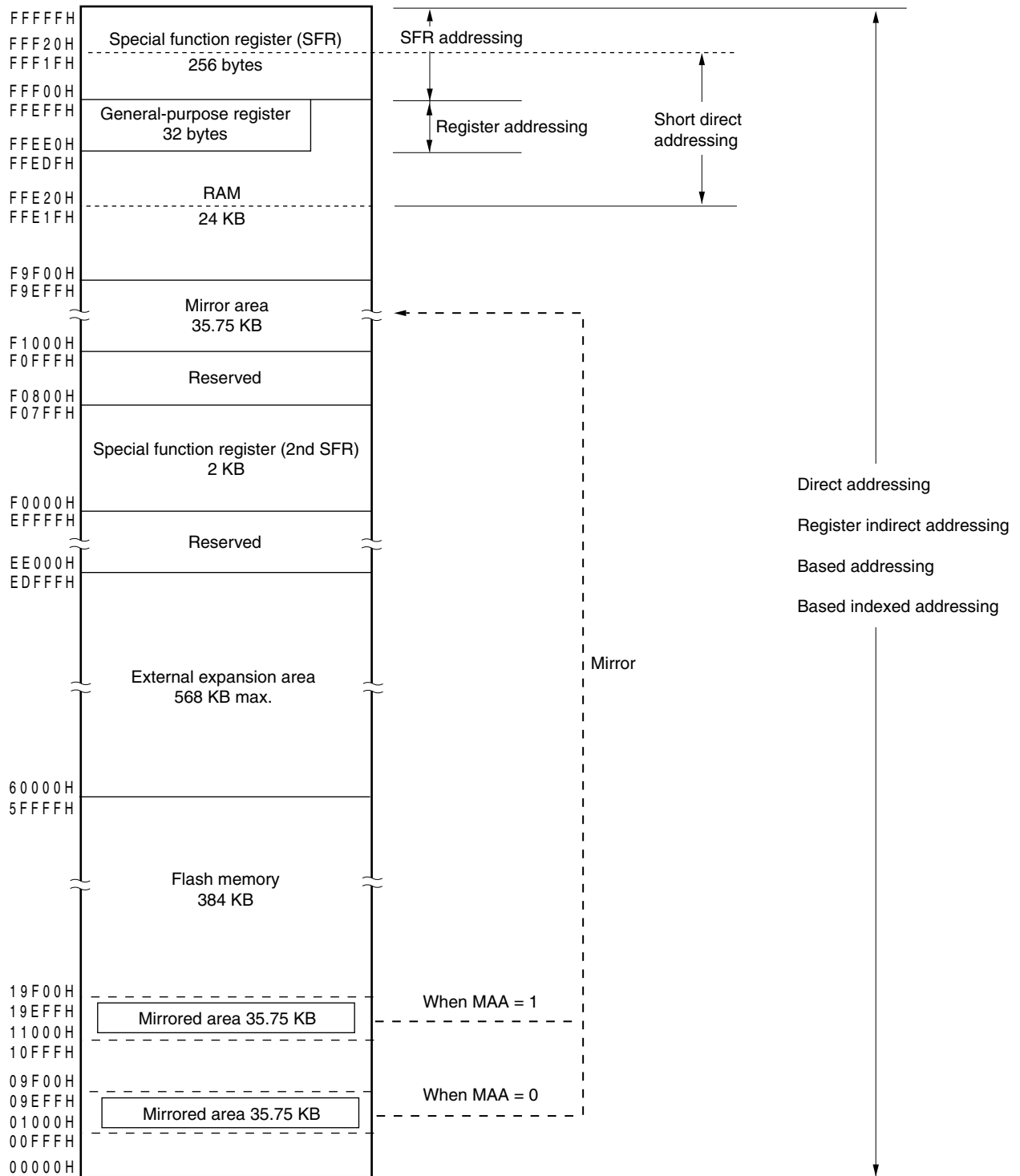
Figure 3-10. Correspondence Between Data Memory and Addressing ( \mu PD78F1177, 78F1177A)
