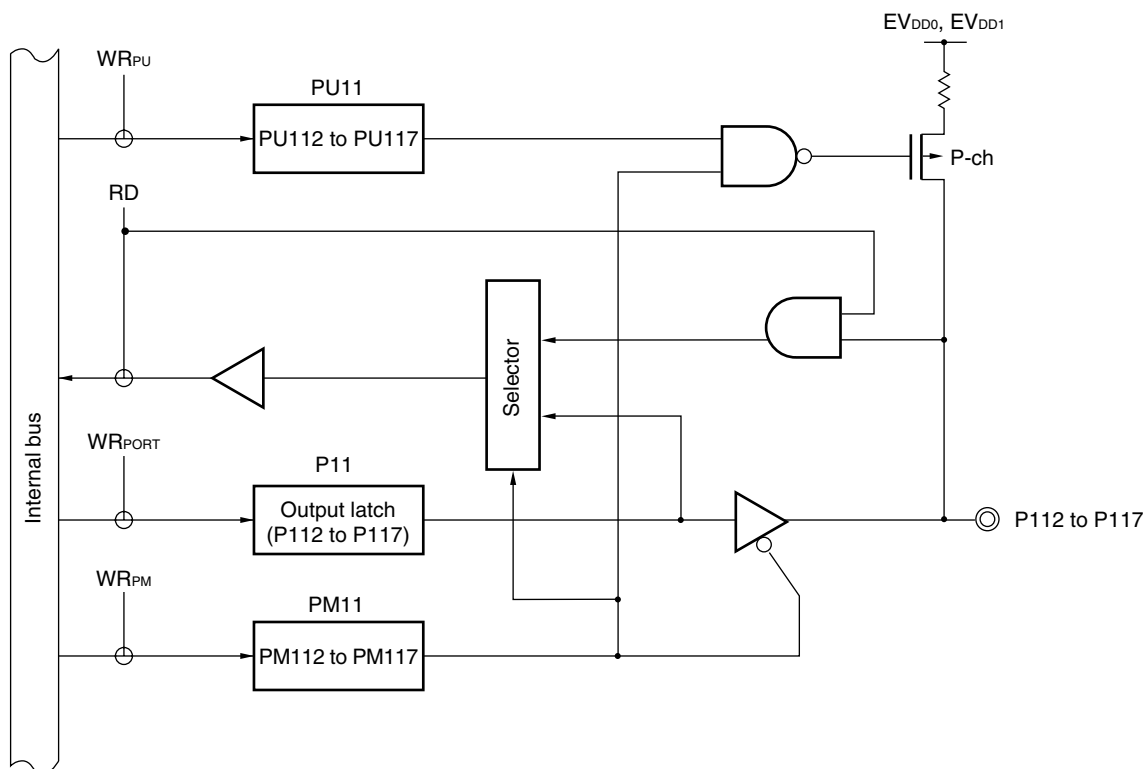
Figure 4-37. Block Diagram of P112 to P117
