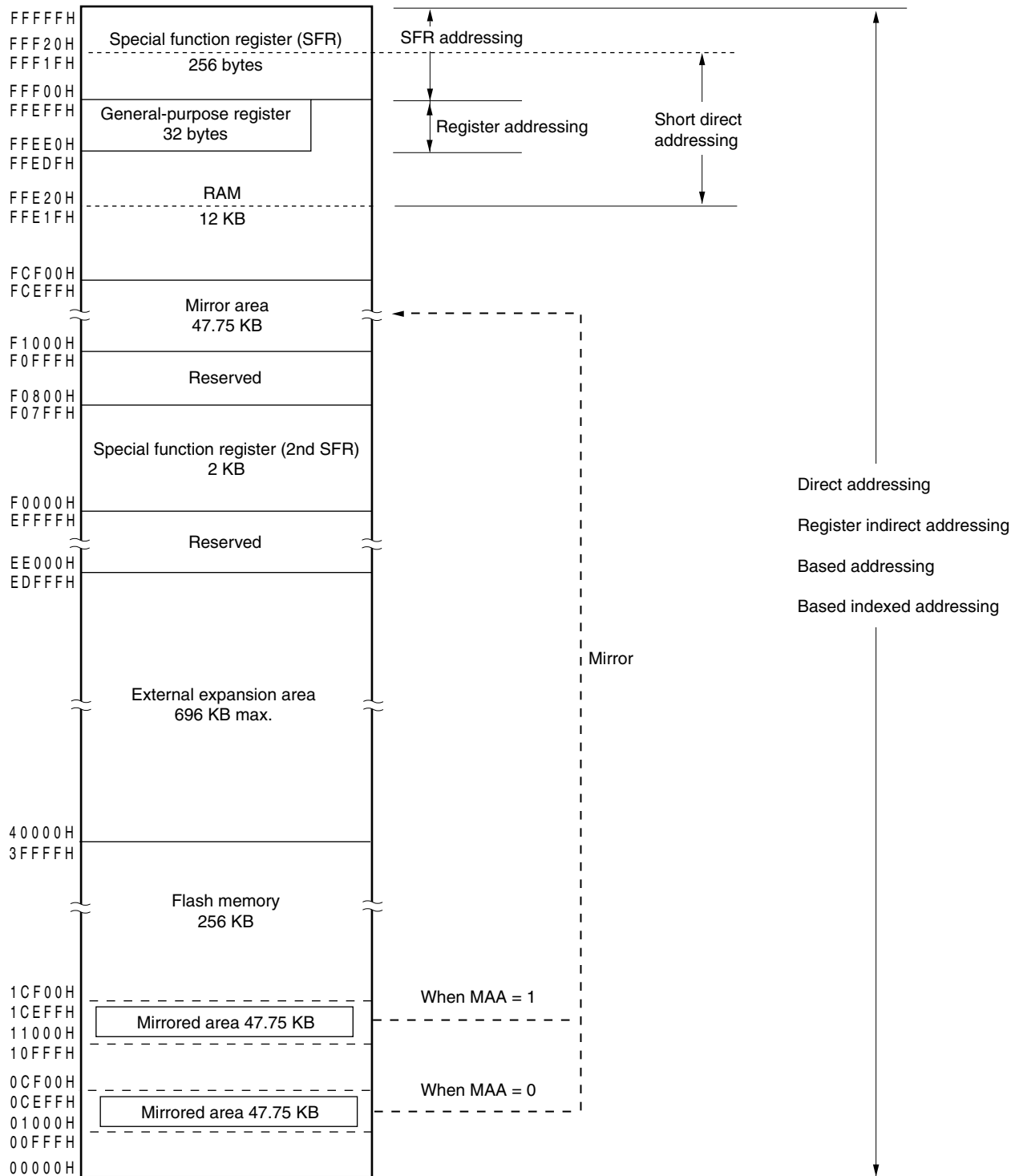
<R> Figure 3-9. Correspondence Between Data Memory and Addressing ( \mu PD78F1176, 78F1176A)
