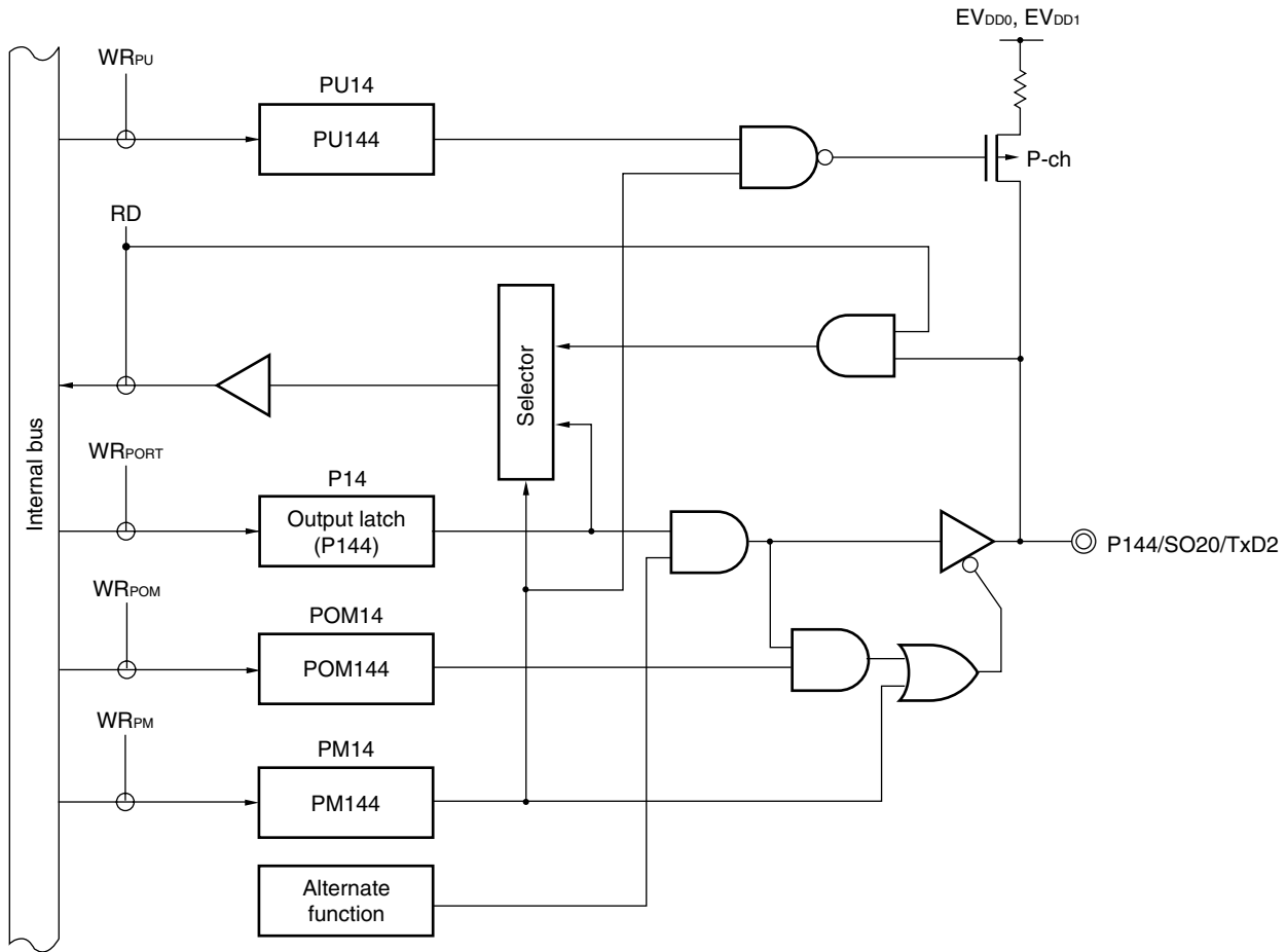
Figure 4-47. Block Diagram of P144
