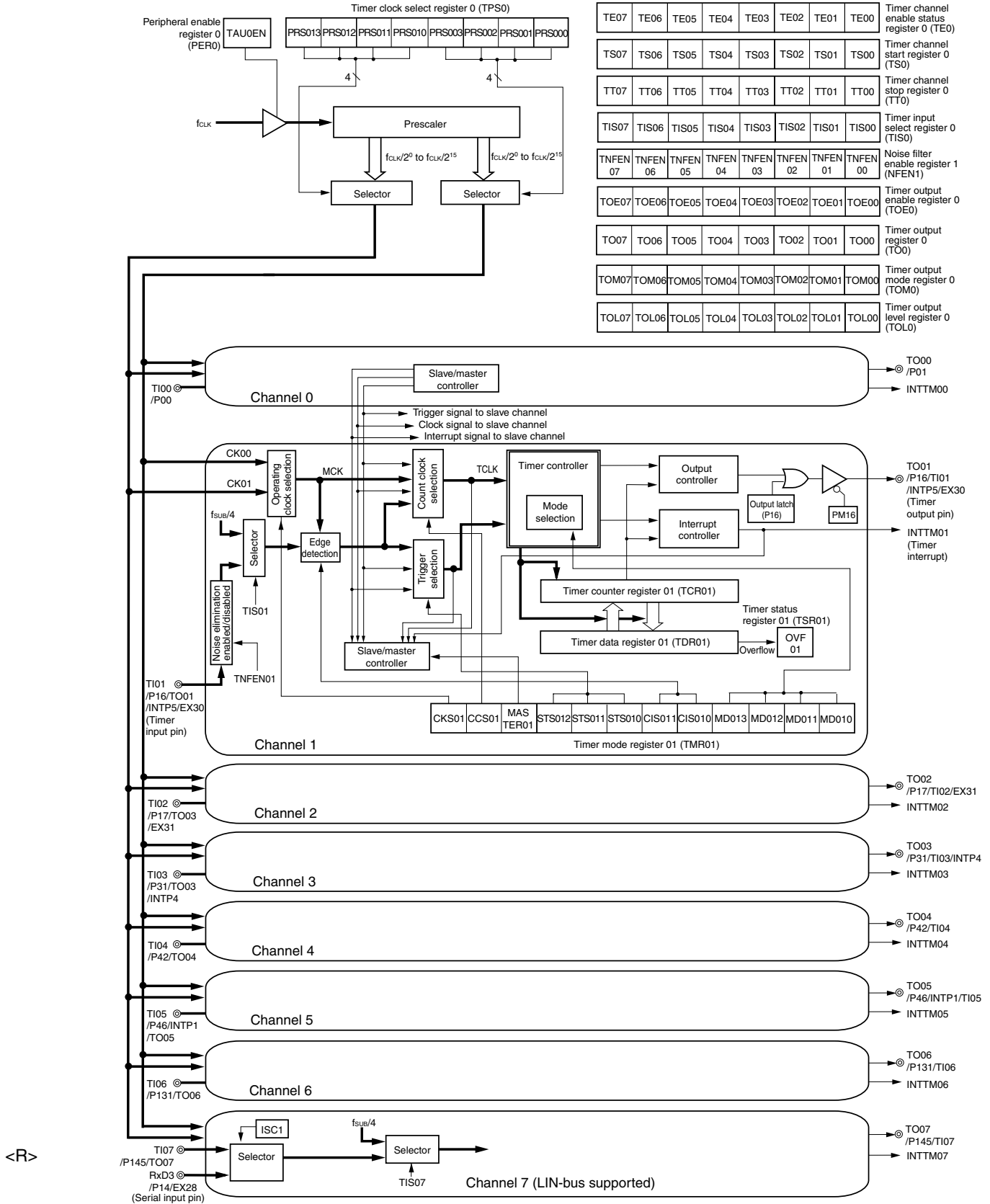
Figure 7-1. Block Diagram of Timer Array Unit 0
