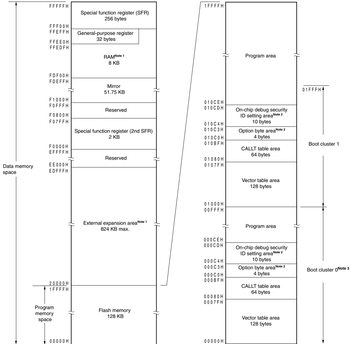
Figure 3-1. Memory Map ( \mu PD78F1174, 78F1174A)
