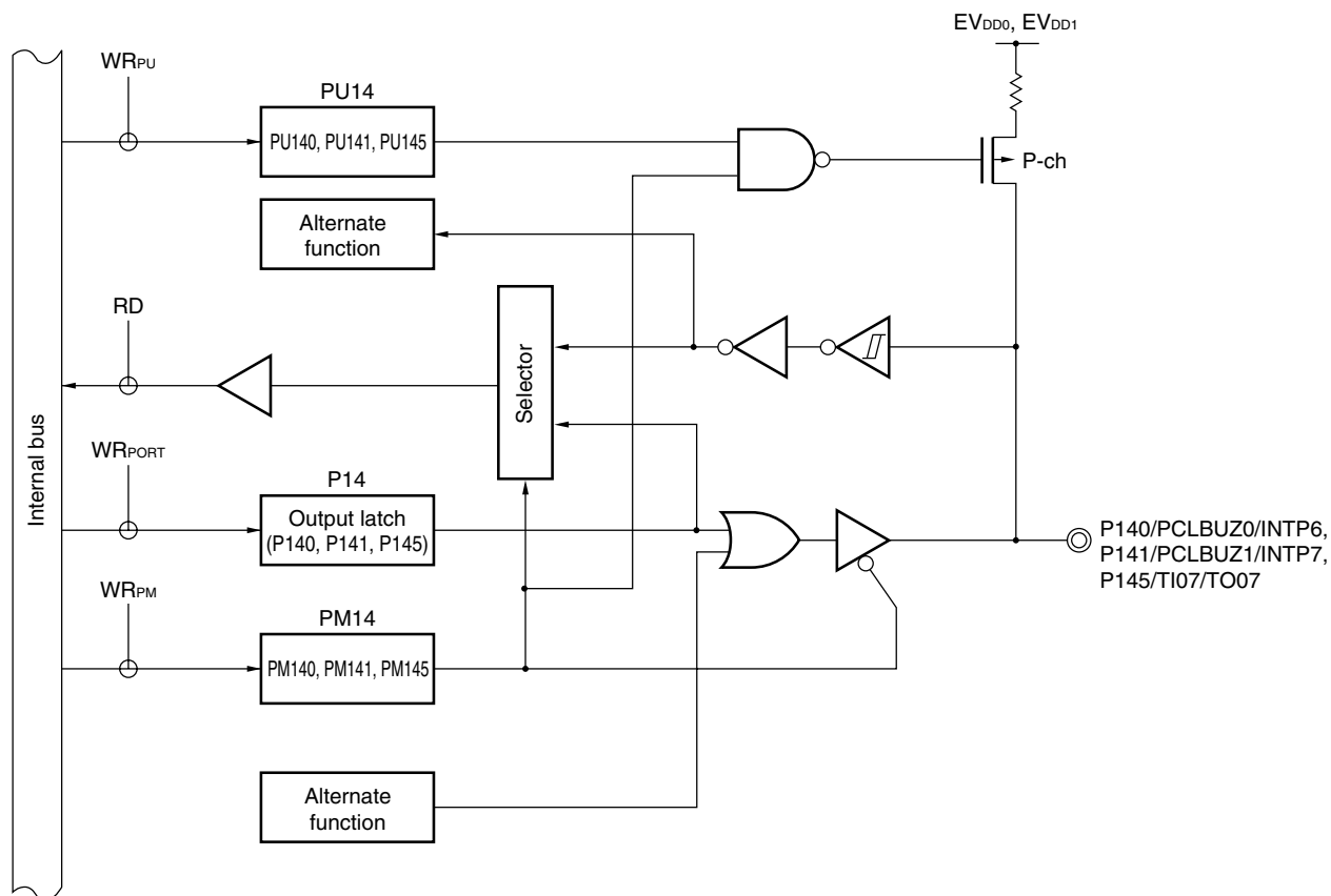
Figure 4-45. Block Diagram of P140, P141, and P145
