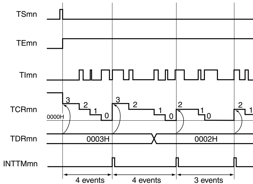
Figure 7-42. Example of Basic Timing of Operation as External Event Counter
