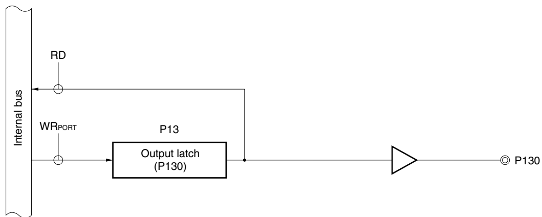
Figure 4-43. Block Diagram of P130
