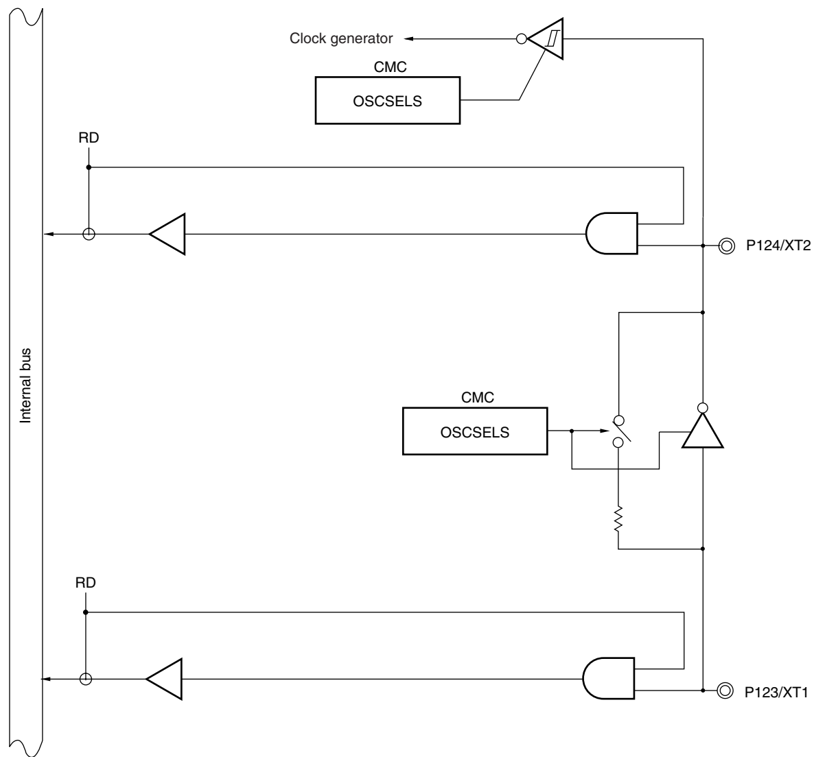
Figure 4-40. Block Diagram of P123 and P124
