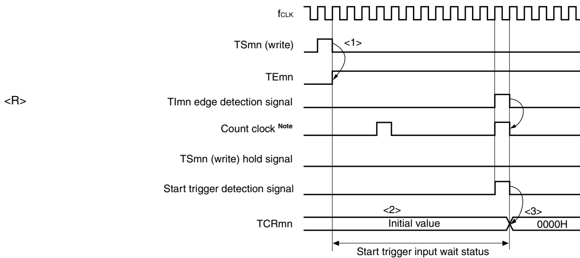
Figure 7-15. Start Timing (In Capture & One-count Mode)
