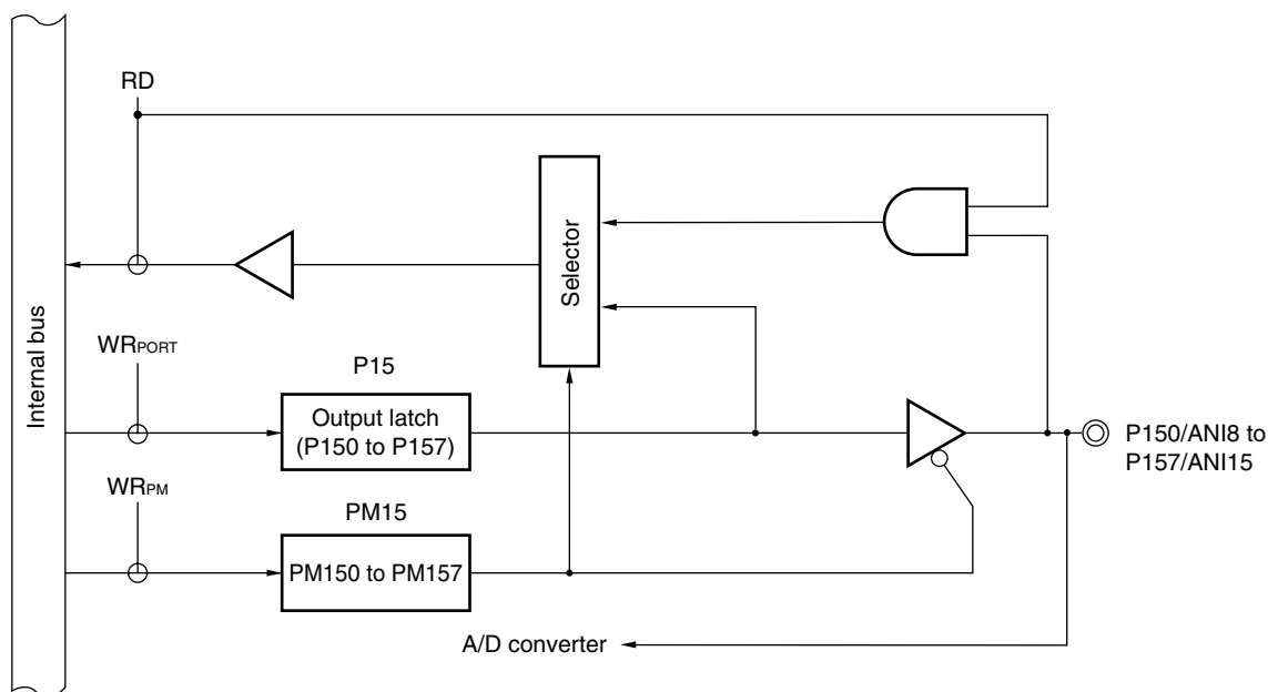
Figure 4-48. Block Diagram of P150 to P157
