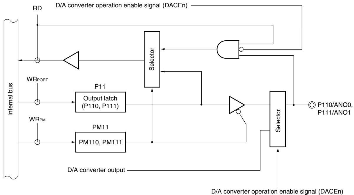
Figure 4-36. Block Diagram of P110 and P111
