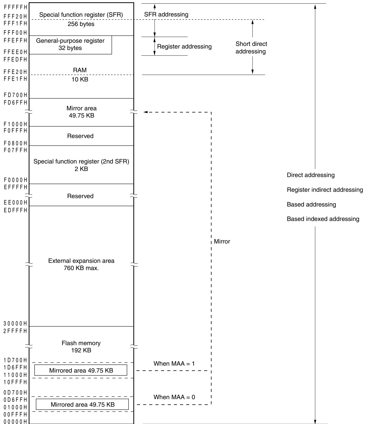
Figure 3-8. Correspondence Between Data Memory and Addressing ( \mu PD78F1175, 78F1175A)
