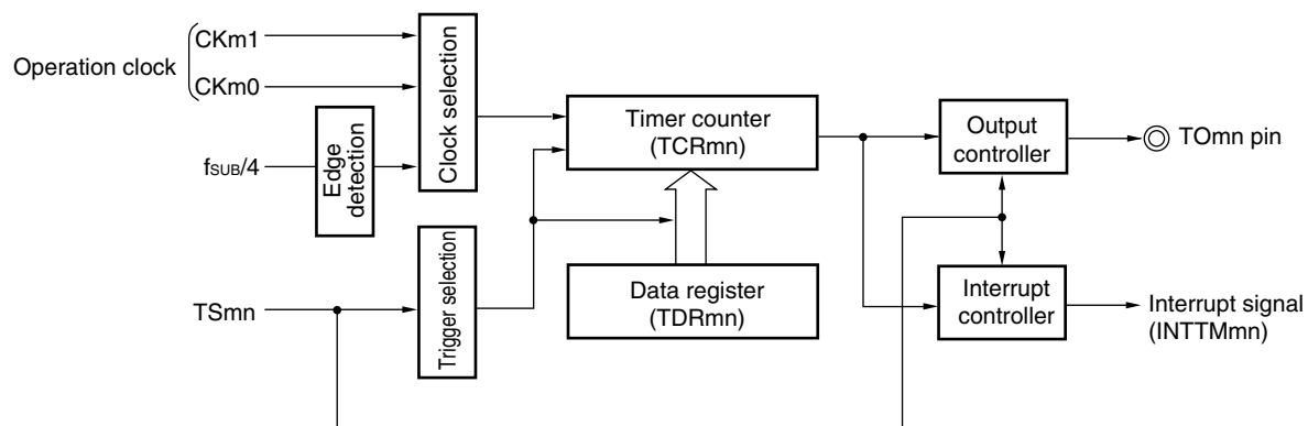
Figure 7-37. Block Diagram of Operation as Interval Timer/Square Wave Output
