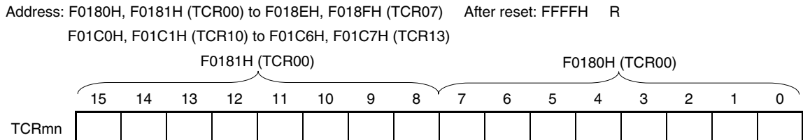
Figure 7-3. Format of Timer/Counter Register mn (TCRmn)
