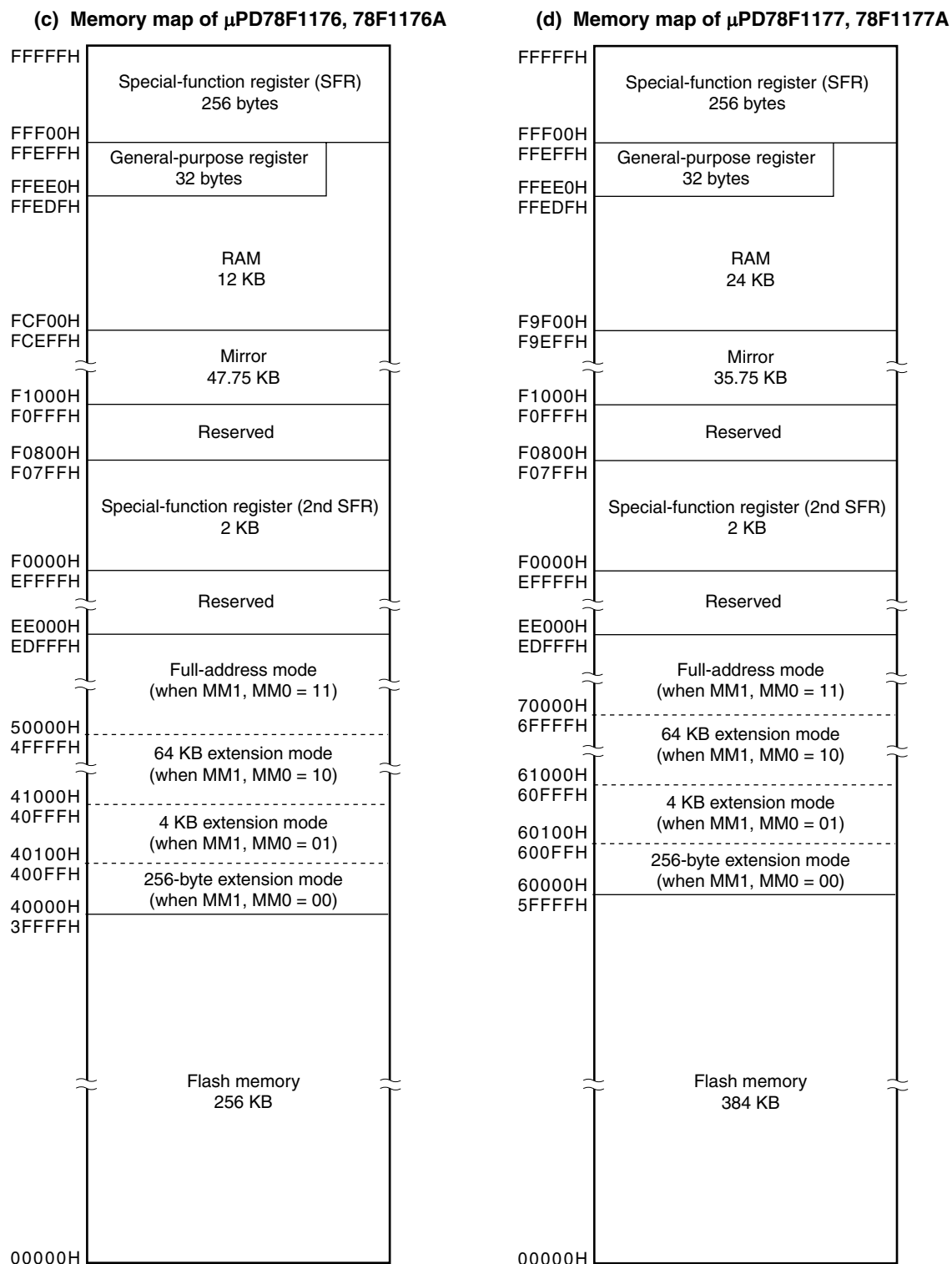
Figure 5-1. Memory Map When Using External Bus Interface Function (2/3)
