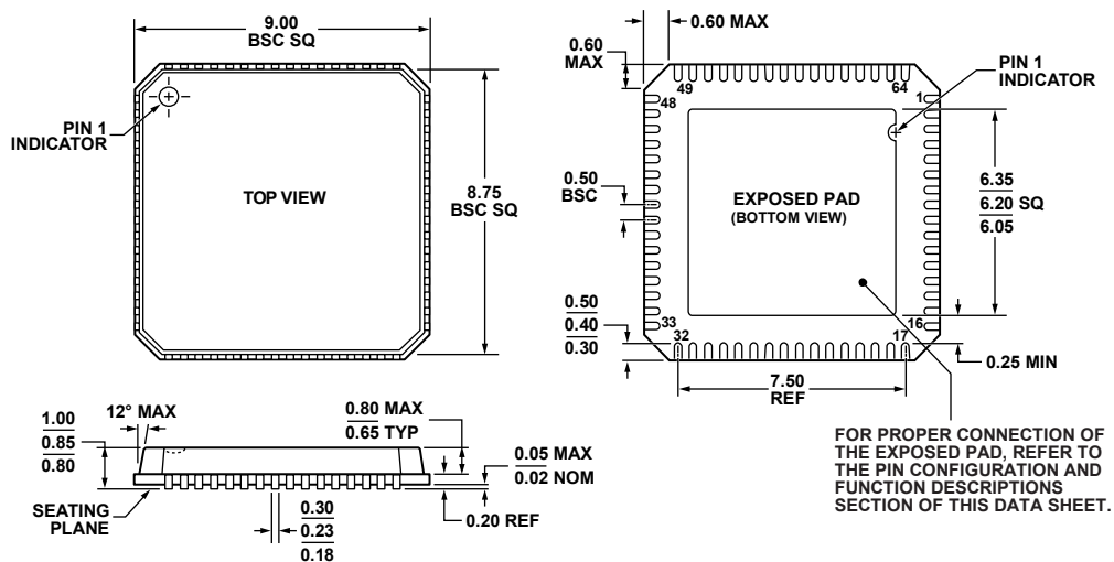
Figure 63. 64-Lead Lead Frame Chip Scale Package [LFCSP_VQ]
