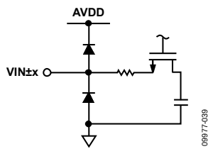
Figure 34. Equivalent Analog Input Circuit
