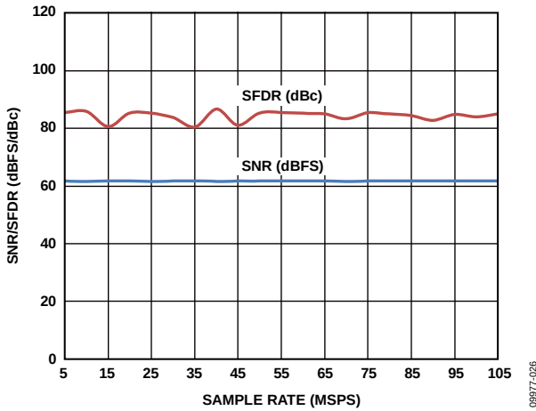
Figure 29. SNR/SFDR vs. Sample Rate with AIN = 9.7 MHz
