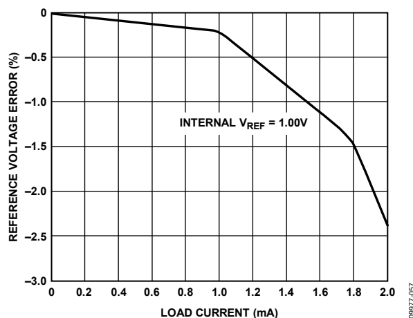
Figure 50. V_{REF} Accuracy vs. Load Current
