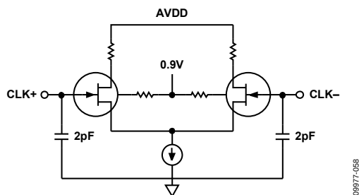
Figure 52. Equivalent Clock Input Circuit
