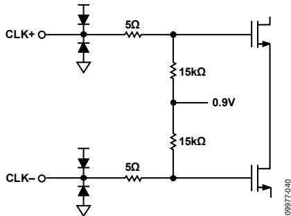
Figure 35. Equivalent Clock Input Circuit
