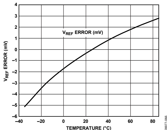
Figure 51. Typical V_{REF} Drift
