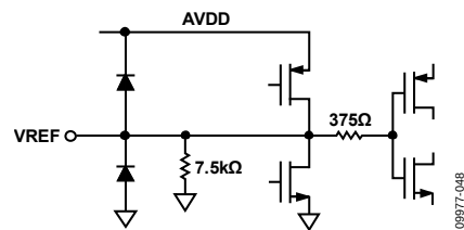
Figure 41. Equivalent VREF Circuit
