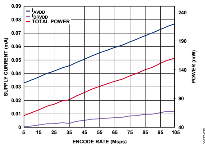
Figure 61. AD9608-105 Power and Current vs. Clock Rate (1.8 V CMOS Output Mode)
