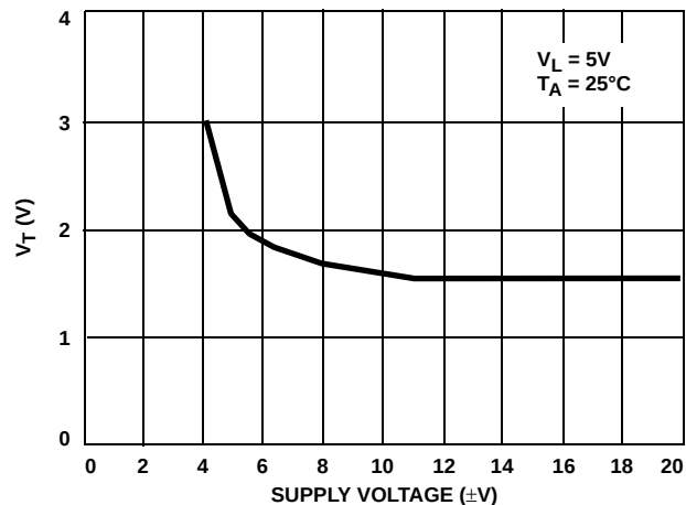
FIGURE 11. INPUT SWITCHING THRESHOLD vs POWER SUPPLY VOLTAGE
