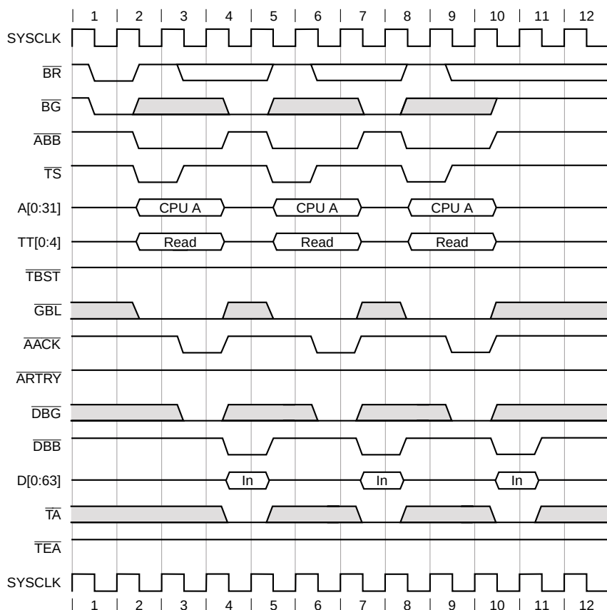
Figure 9-12. Fastest Single-Beat Reads
