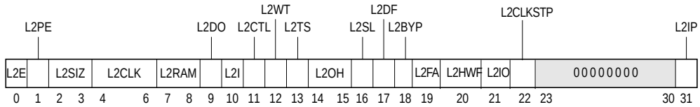
Figure 2-7. L2 Cache Control Register (L2CR)
