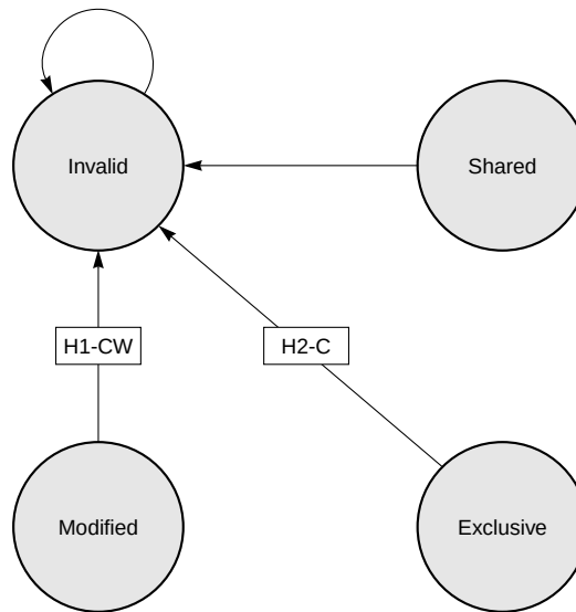
Figure 3-14. RWITM Transaction—MPX Bus Mode, L1_INTVEN = 0b110
