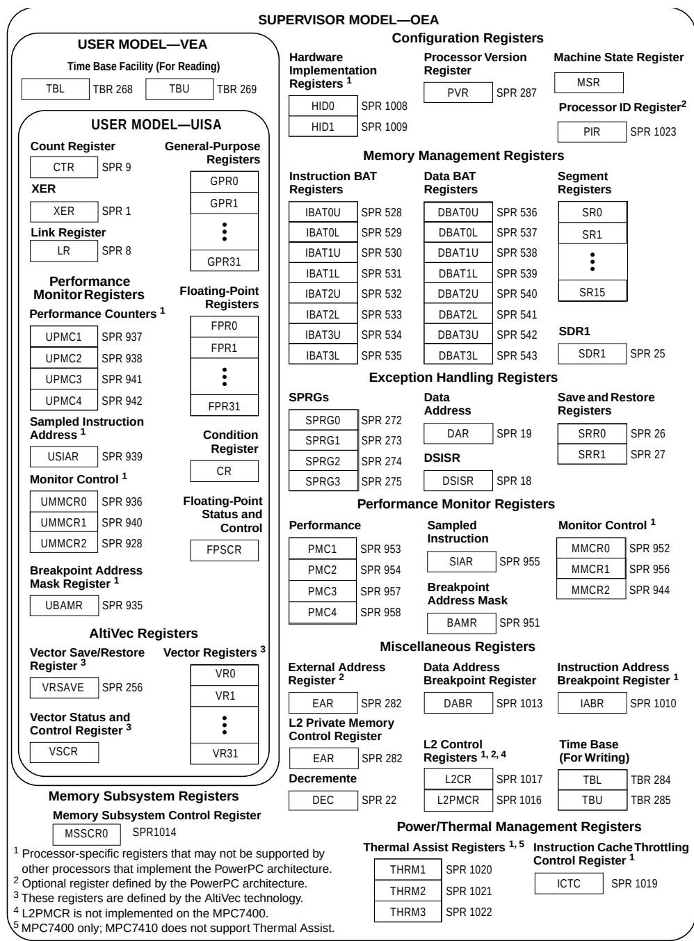
Figure 1-5. MPC7410 Microprocessor Programming Model—Registers
