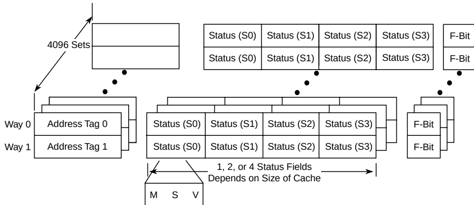
Figure 3-35. L2 Cache Controller Tag Organization
