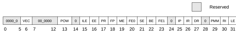
Figure 2-2. Machine State Register (MSR)
