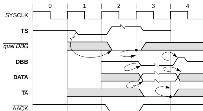
Figure 9-9. Normal Single-Beat Write Termination
