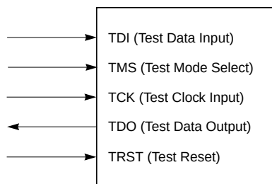
Figure 9-28. IEEE 1149.1a-1993 Compliant Boundary-Scan Interface
