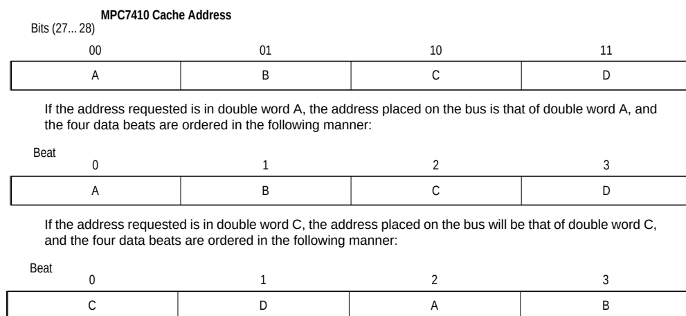
Figure 3-39. Double-Word Address Ordering—Critical Double Word First
