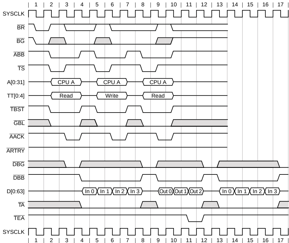
Figure 9-17. Use of Transfer Error Acknowledge ( \overline{\text{TEA}} )
