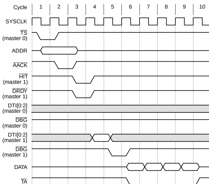
Figure 9-25. Data-Only Transaction for a Flush Operation
