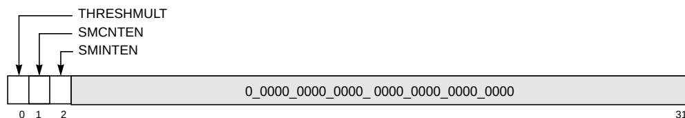
Figure 2-14. Monitor Mode Control Register 2 (MMCR2)
