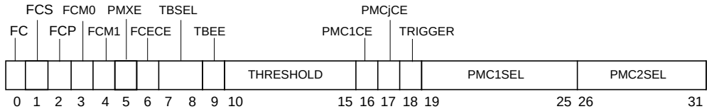
Figure 2-12. Monitor Mode Control Register 0 (MMCR0)
