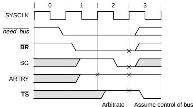
Figure 9-18. MPX Bus Address Bus Arbitration—Non-Parked Case
