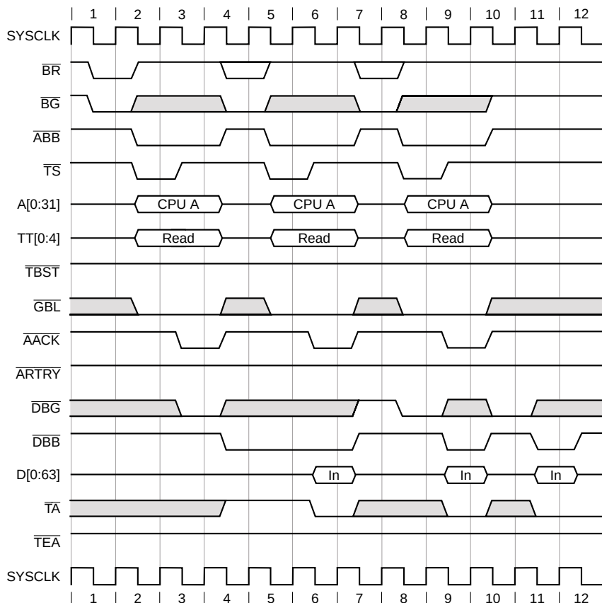
Figure 9-14. Single-Beat Reads Showing Data-Delay Controls
