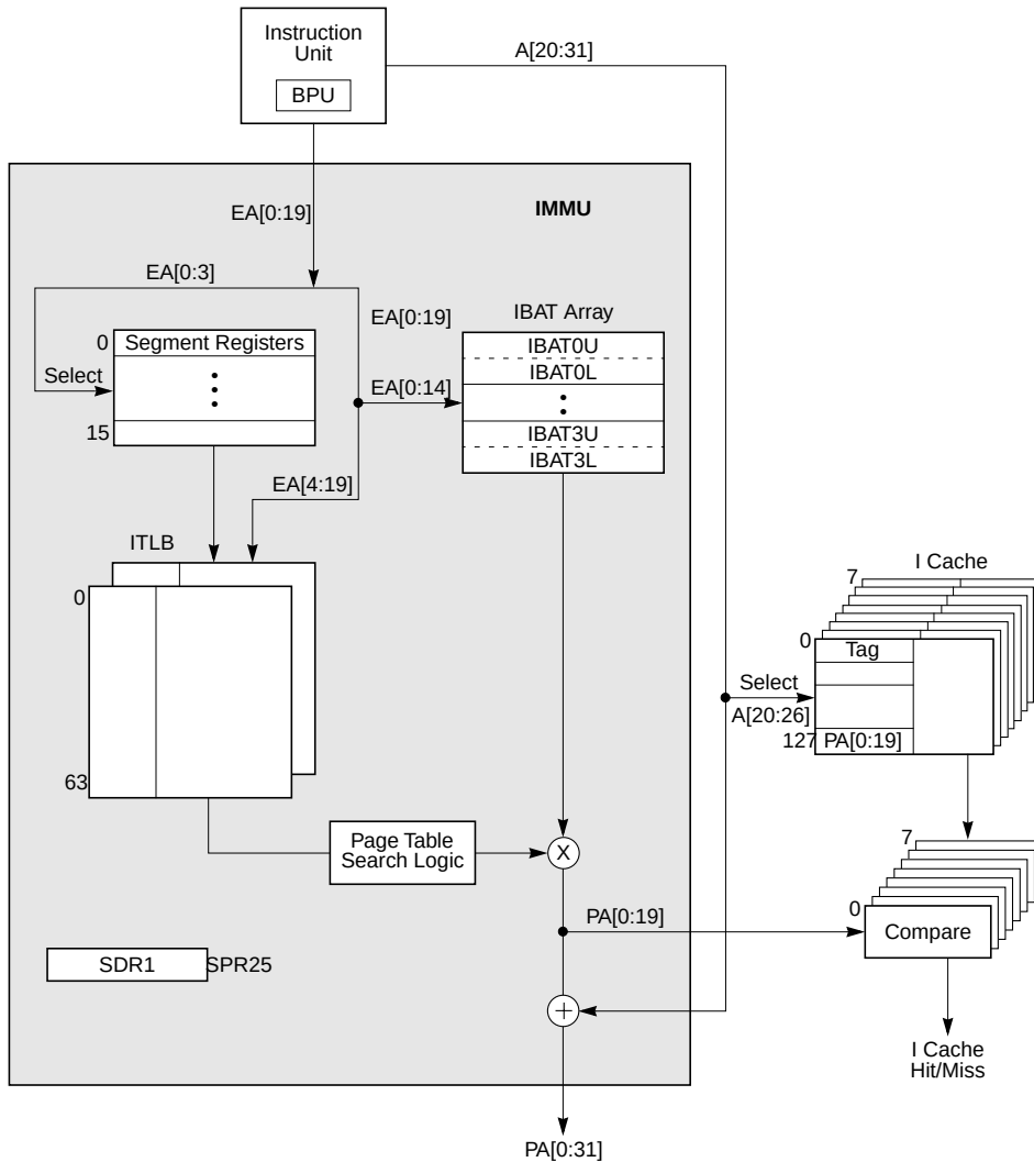
Figure 5-2. MPC7410 Microprocessor IMMU Block Diagram
