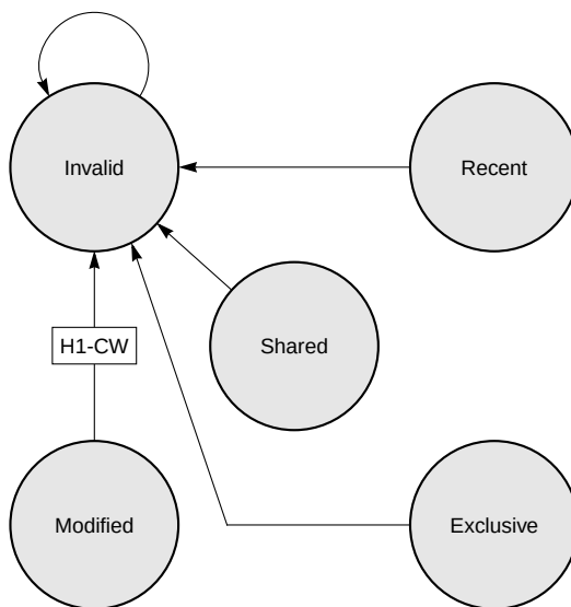
Figure 3-22. Flush Transaction—MPX Bus Mode, L1_INTVEN = 0b111
