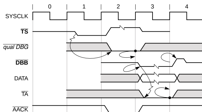
Figure 9-8. Normal Single-Beat Read Termination
