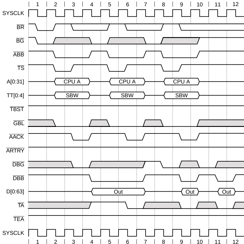
Figure 9-15. Single-Beat Writes Showing Data Delay Controls
