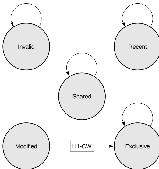
Figure 3-23. Clean Transaction—MPX Bus Mode, L1_INTVEN = 0b111
