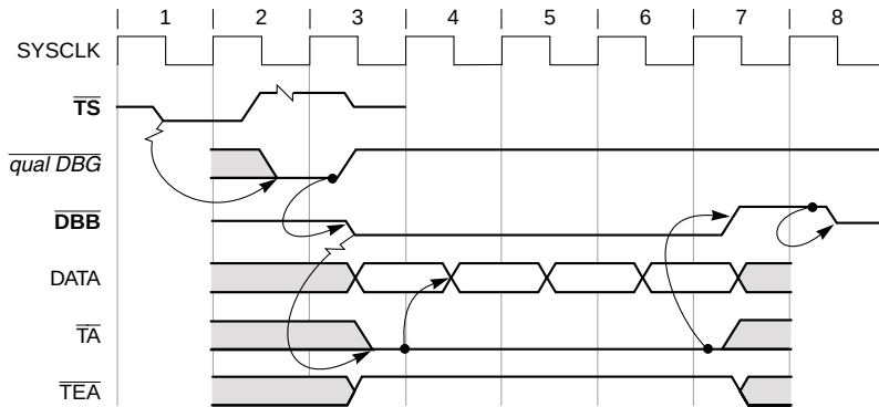
Figure 9-10. Normal Burst Transaction
