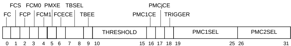
Figure 11-1. Monitor Mode Control Register 0 (MMCR0)
