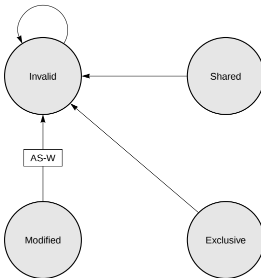
Figure 3-10. Write Transaction—MPX Bus Mode, L1_INTVEN = 0b100
