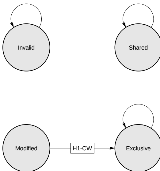
Figure 3-17. Clean Transaction—MPX Bus Mode, L1_INTVEN = 0b110
