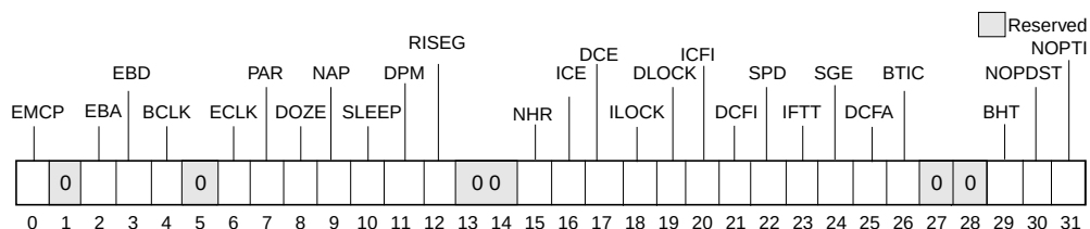
Figure 2-3. Hardware Implementation-Dependent Register 0 (HID0)
