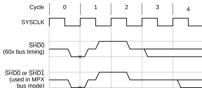
Figure 9-22. \overline{\text{SHD0}} and \overline{\text{SHD1}} Negation Timing
