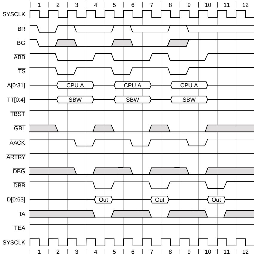
Figure 9-13. Fastest Single-Beat Writes
