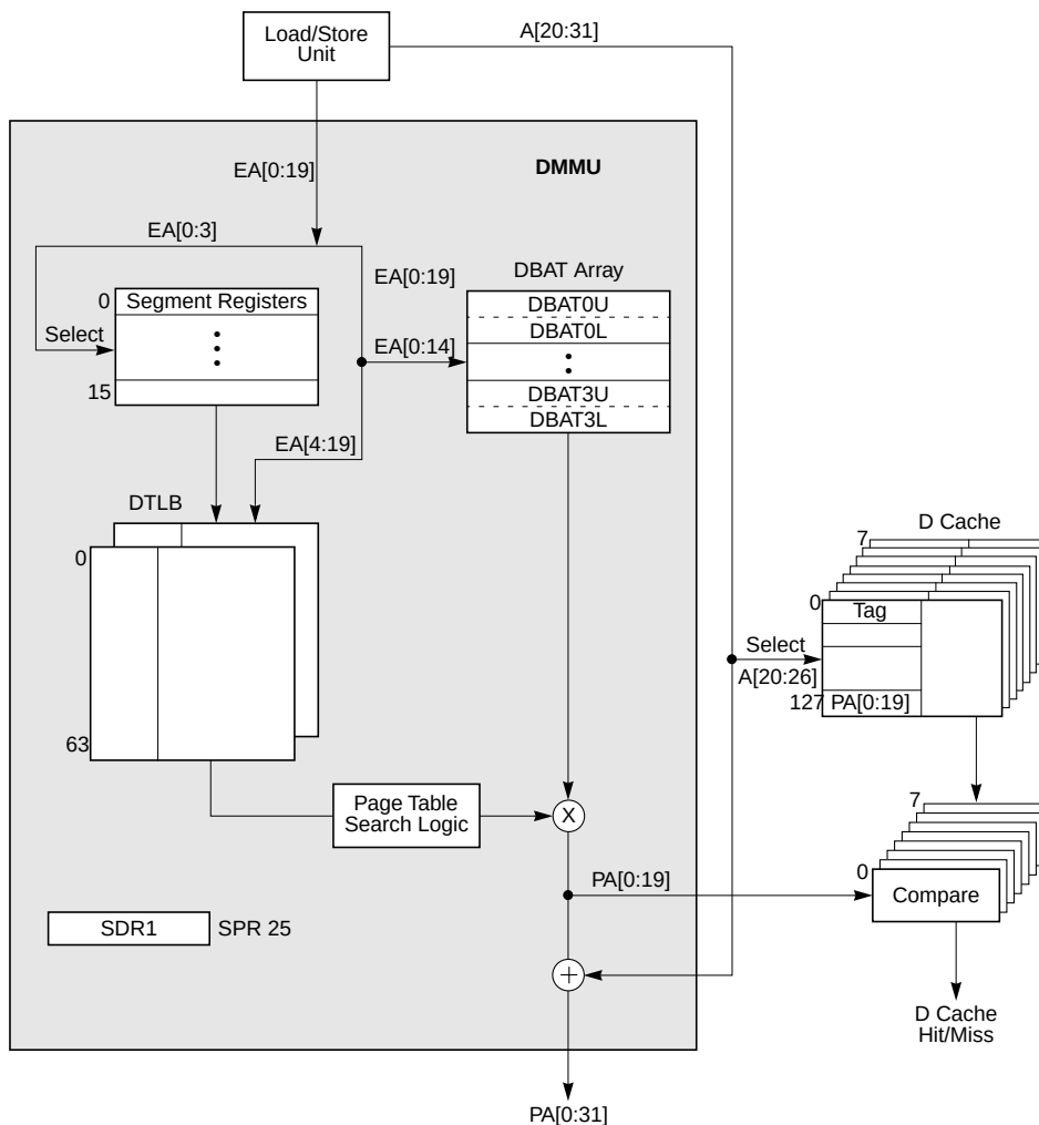
Figure 5-3. MPC7410 Microprocessor DMMU Block Diagram
