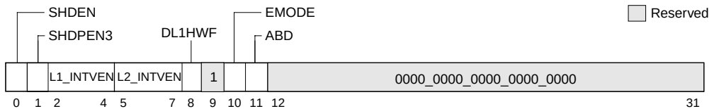
Figure 2-5. Memory Subsystem Control Register (MSSCR0)
