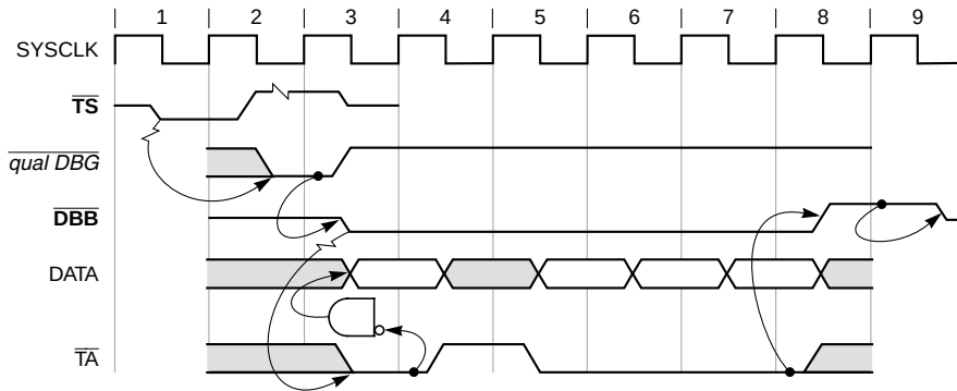
Figure 9-11. Read Burst with \overline{TA} Wait States
