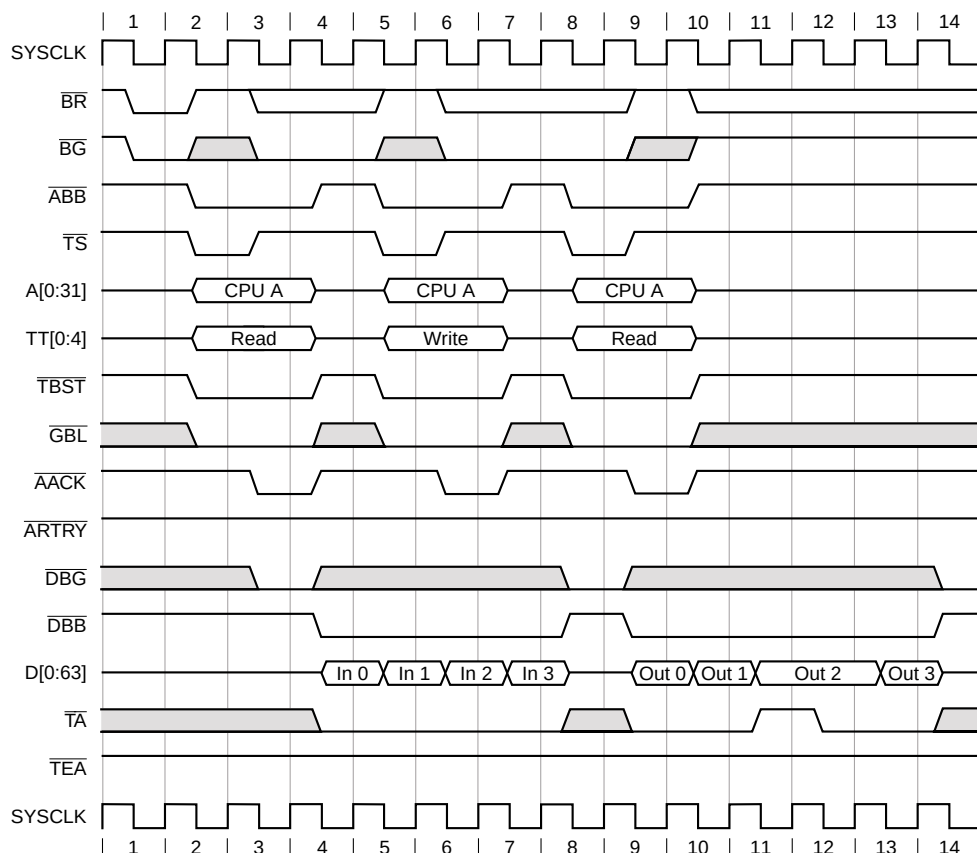
Figure 9-16. Burst Transfers with Data Delay Controls
