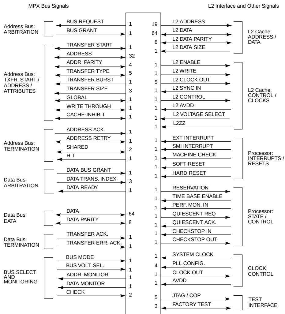
Figure 1-4. MPC7410 Microprocessor Signal Groups
