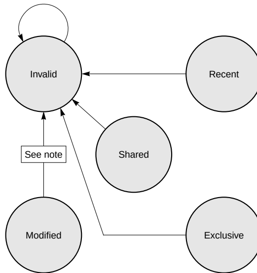
Figure 3-24. Kill Transaction—MPX Bus Mode, L1_INTVEN = 0b111
