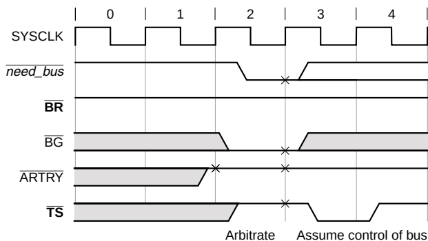
Figure 9-19. Bus Arbitration—Parked Case
