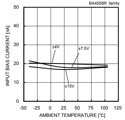
Fig. 34 Input Bias Current - Ambient Temperature (Vcm=0[V], Vout=0[V])
