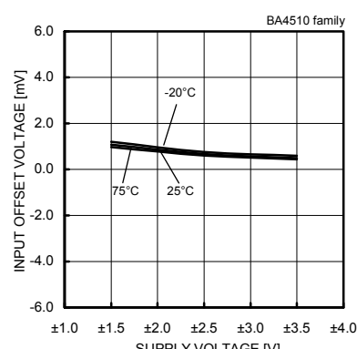
Fig. 273 Input Offset Voltage - Supply Voltage (V icm =0[V], V out =0[V])
