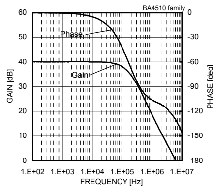
Fig. 287 Voltage Gain - Frequency (V CC /V EE =2.5[V]/-2.5[V], A v =40[dB], R L =10[kΩ])
