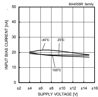
Fig. 33 Input Bias Current - Supply Voltage (Vcm=0[V], Vout=0[V])
