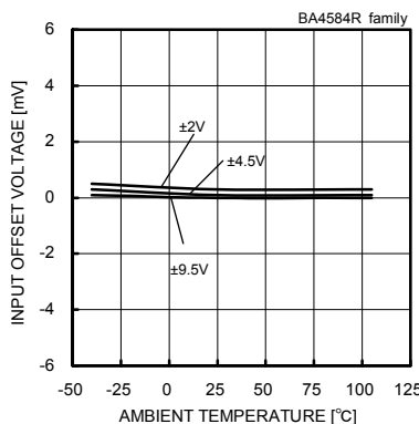
Fig. 164 Input Offset Voltage - Ambient Temperature (V icm =0[V], V out =0[V])
