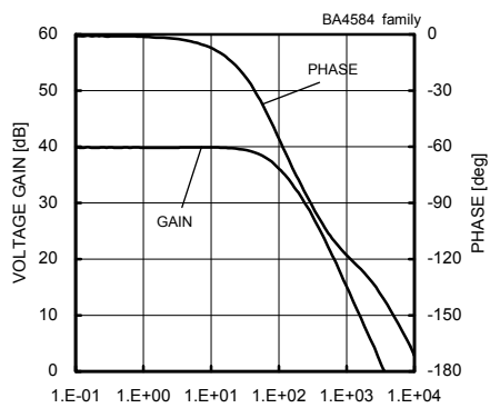
Fig. 154 Voltage Gain - Frequency ( V_{CC}/V_{EE}=+15[V]/-15[V] , A_v=40[dB] , R_L=2[k\Omega] , T_a=25[^\circ C] )
