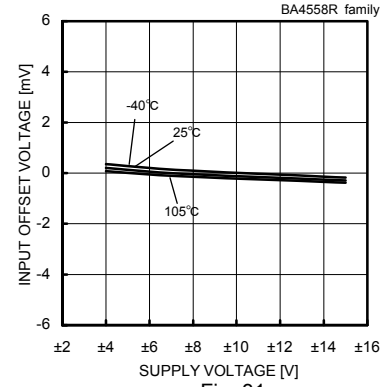
Fig. 31 Input Offset Voltage - Supply Voltage (Vcm=0[V], Vout=0[V])
