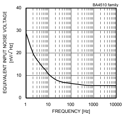
Fig. 286 Equivalent Input Noise Voltage - Frequency (V CC /V EE =2.5[V]/-2.5[V])
