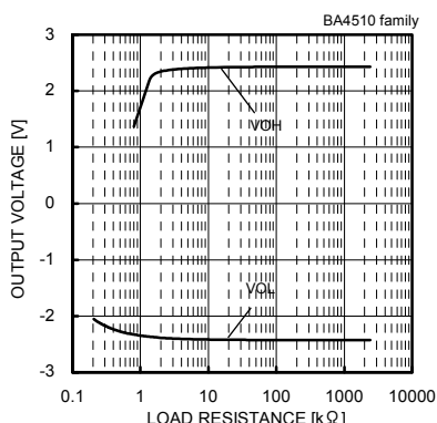
Fig. 268 Maximum Output Voltage Swing - Load Resistance (VCC/VEE=2.5[V]/-2.5[V], Ta=25[°C])
