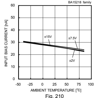
Input Bias Current - Ambient Temperature (Vcm=0[V], Vout=0[V])
