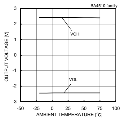
Fig. 270 Maximum Output Voltage - Ambient Temperature (VCC/VEE=2.5[V]/-2.5[V], RL=10[kΩ])
