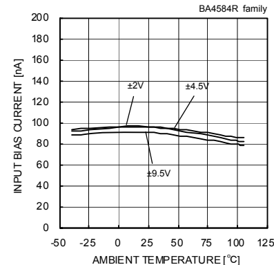
Fig. 166 Input Bias Current - Ambient Temperature (V icm =0[V], V out =0[V])
