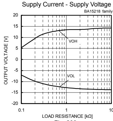
Maximum Output Voltage - Load Resistance (VCC/VEE=+15[V]/-15[V], Ta=25[°C])
