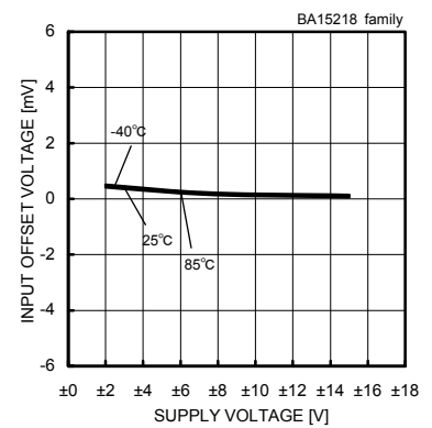
Input Offset Voltage - Supply Voltage (Vcm=0[V], Vout=0[V])
