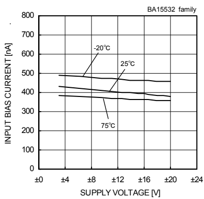
Fig. 253 Input Bias Current - Supply Voltage (Vicm=0[V], Vout=0[V])
