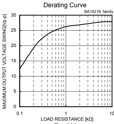
Maximum Output Voltage Swing - Load Resistance (VCC/VEE=+15[V]/-15[V], Ta=25[°C])
