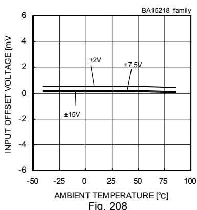
Input Offset Voltage - Ambient Temperature (Vcm=0[V], Vout=0[V])
