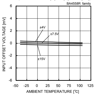
Fig. 32 Input Offset Voltage - Ambient Temperature (Vcm=0[V], Vout=0[V])
