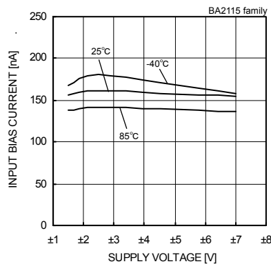
Fig. 298 Input Bias Current - Supply Voltage (Vicm=0[V], Vout=0[V])
