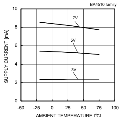
Fig. 267 Supply Current - Ambient Temperature
