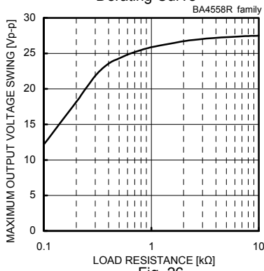
Fig. 26 Maximum Output Voltage Swing - Load Resistance (VCC/VEE=+15[V]/-15[V], Ta=25[°C])
