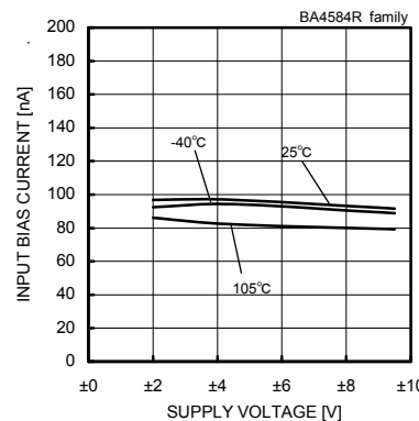
Fig. 165 Input Bias Current - Supply Voltage (V icm =0[V], V out =0[V])
