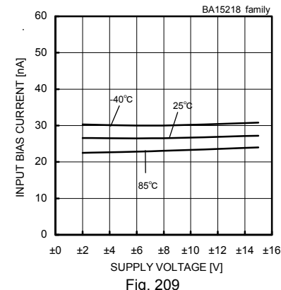
Input Bias Current - Supply Voltage (Vcm=0[V], Vout=0[V])
