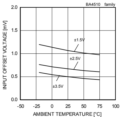
Fig. 274 Input Offset Voltage - Ambient Temperature (V icm =0[V], V out =0[V])
