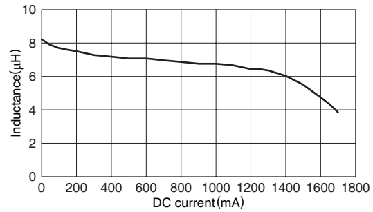
VLF5014AT-150MR76
