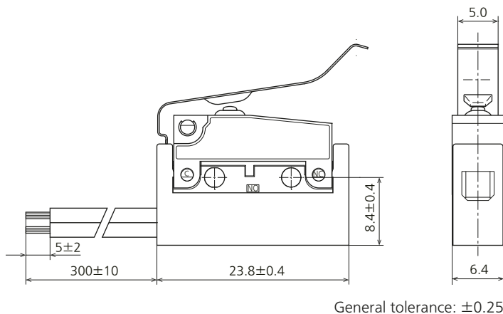
External dimensions
