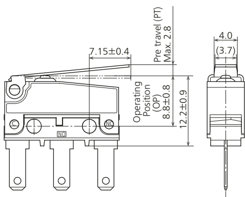
External dimensions
