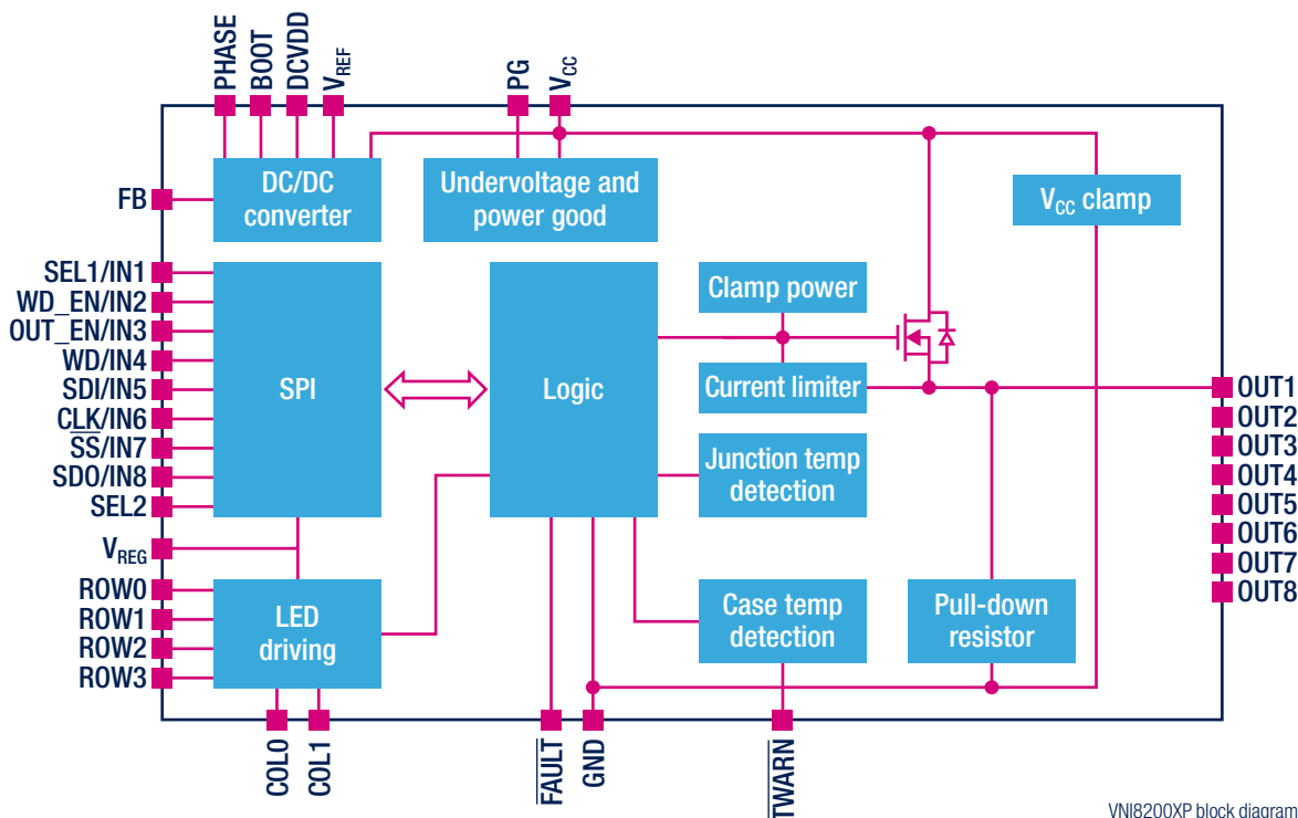
VNI8200XP block diagram
