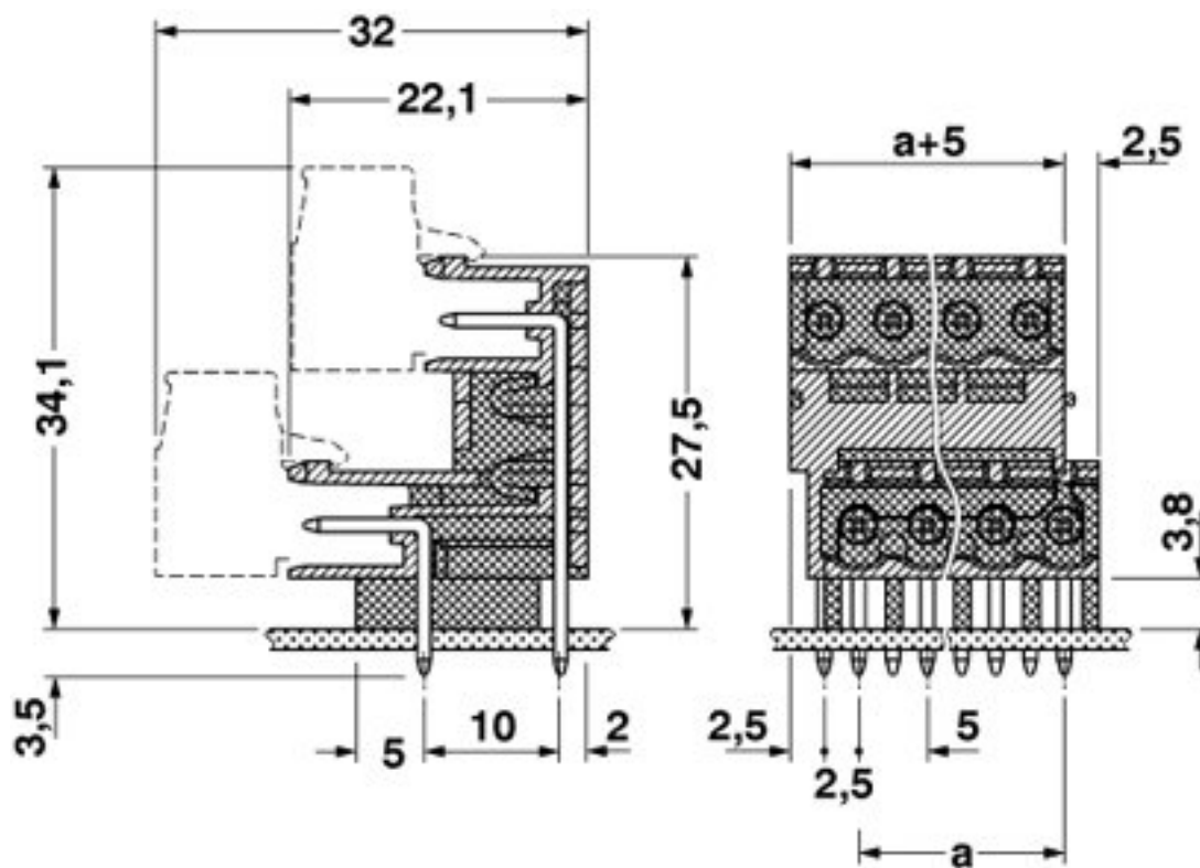
Dimensional drawing
