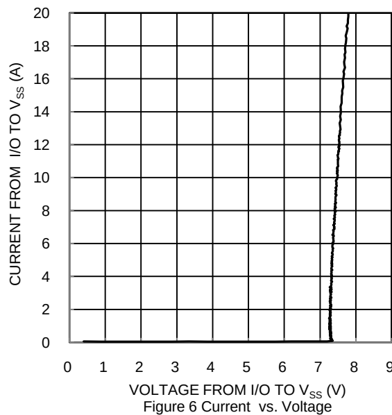
Figure 6 Current vs. Voltage
