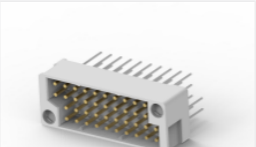
TE Part #825308-1 WIRING CONN 40 POS
