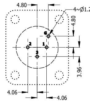
PCB LAYOUT CONNECTOR SIDE
