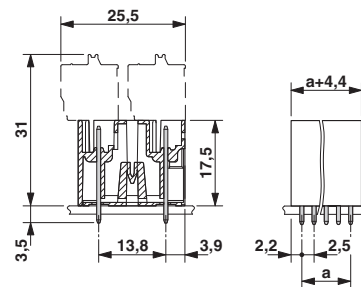
Dimensioned drawing
