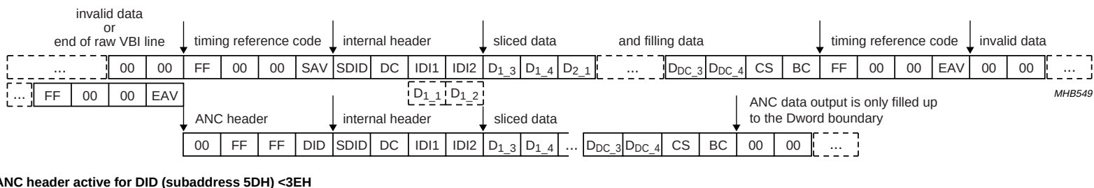
Fig.30 Sliced data formats on the I-port in 8-bit mode.
