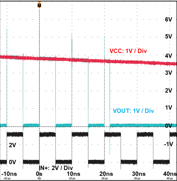
Figure 9. Shutdown Time (0 \Omega as R OUTH and R OUTL , 220 pF load)
