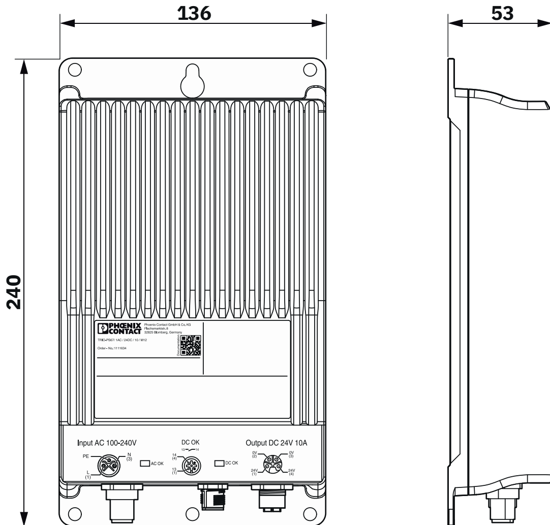
Dimensional drawing
