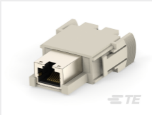
TE Part #T2113000201-200 HMN-RJ45-F CAT6A
