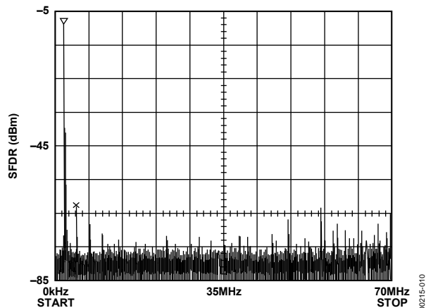
Figure 10. Single-Tone SFDR @ f_{CLK} = 140 \text{ MHz} ( f_{OUT} = 2 \text{ MHz} )
