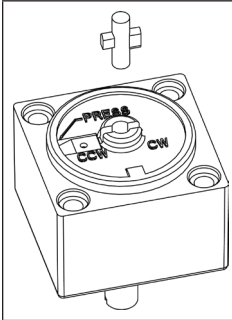
FIGURE 9. EXPLODED VIEW OF CLAMP & SCREW
