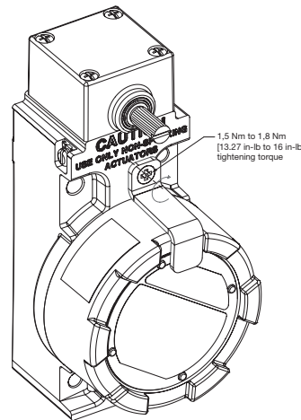
FIGURE 10. WIRING INSTRUCTIONS
