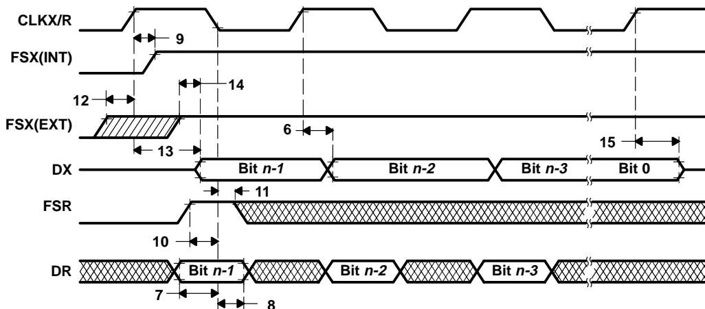
Figure 24. Timing for Fixed Data-Rate Mode
